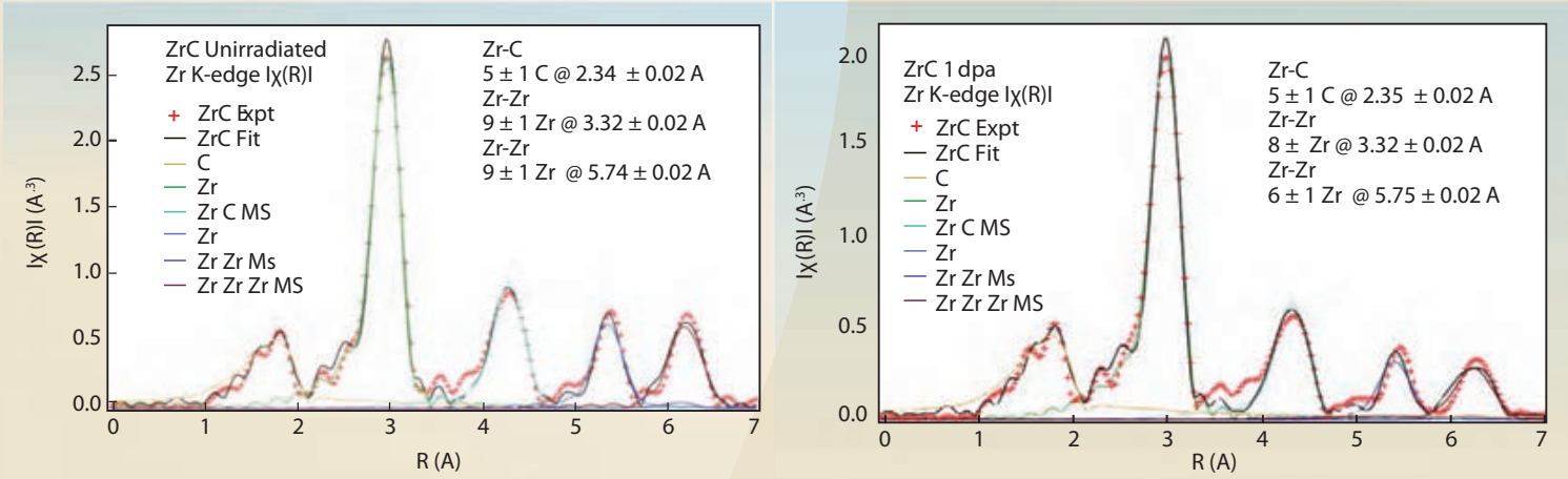
Figure 2. Measurements of ZrC and ZrN show similar results, though shorter interatomic distances were observed for ZrN.
