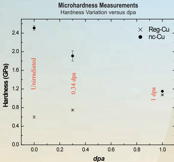
Figure 2. Microhardness measurements of the nanocrystalline copper show radiation-induced hardness variations relative to variations in dosage levels (dpa).
