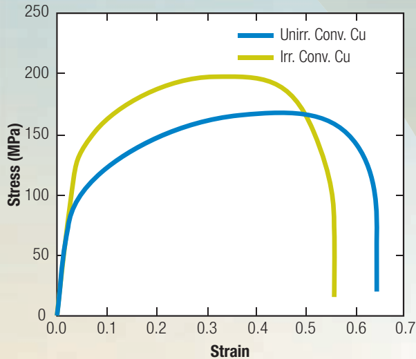
Figure 1. Stress-strain curves for conventional copper (below left) and nanocrystalline copper (below right) show radiation-induced hardening for conventional copper.
