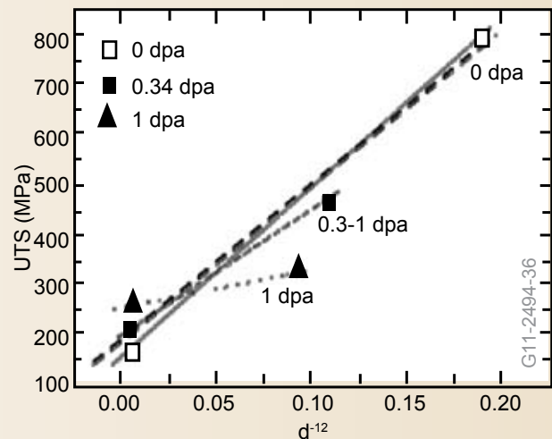
Figure 4. Hall-Petch plot
