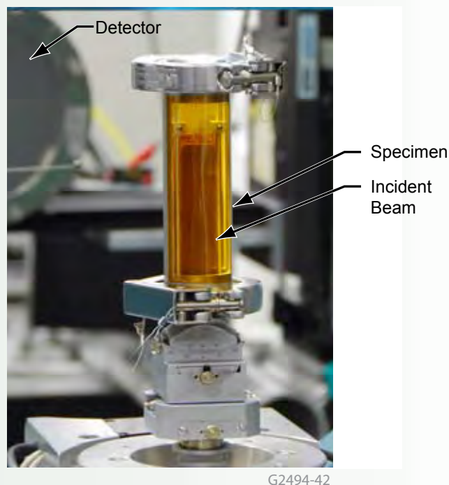
Figure 1. Bare depleted U10Mo foil mounted at beamline 10-ID
