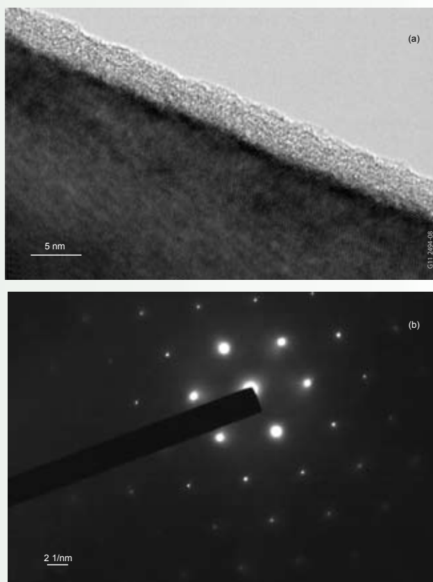
Figure 1. (a) TEM micrograph of a \text{Ti}_2\text{AlN} sample (b) Selected area.
