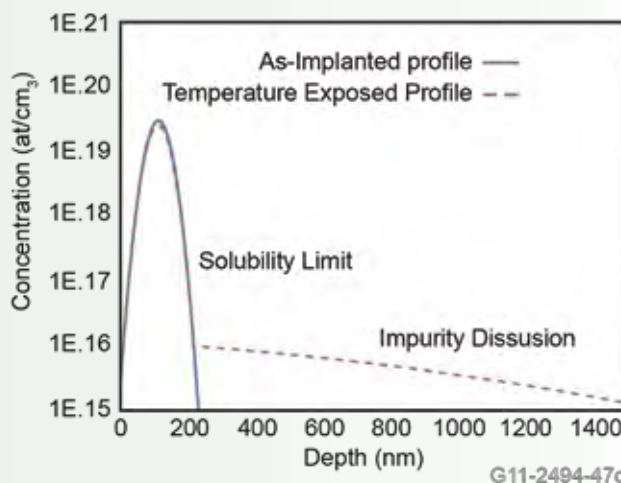
Figure 1. Schematic of an ion implantation diffusion couple depth profile
