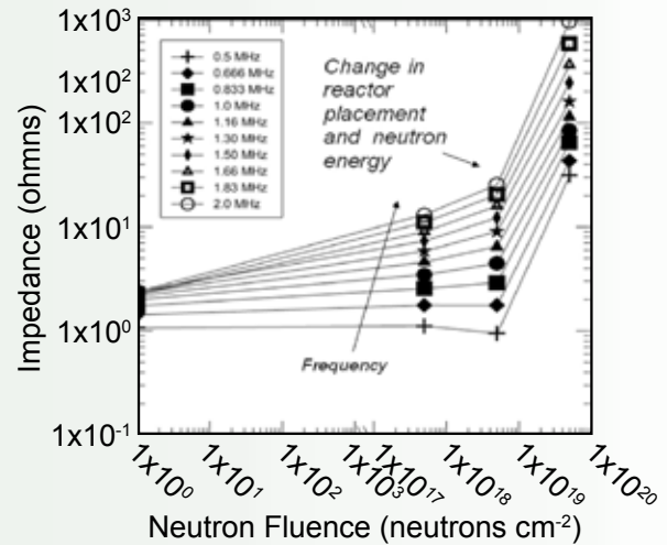
Figure 1: Impedance Results from Silicon Carbide Samples Subjected to Varying Levels of Neutron Fluence.
