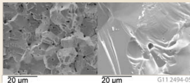
Figure 2. The nonirradiated MgO SEM image (left) shows intergranular fractures through pores on the grain boundaries. The irradiated MgO SEM image (right) shows transgranular fracture, which can be attributed to the irradiation, which caused the grains to become more brittle than the grain boundaries.
