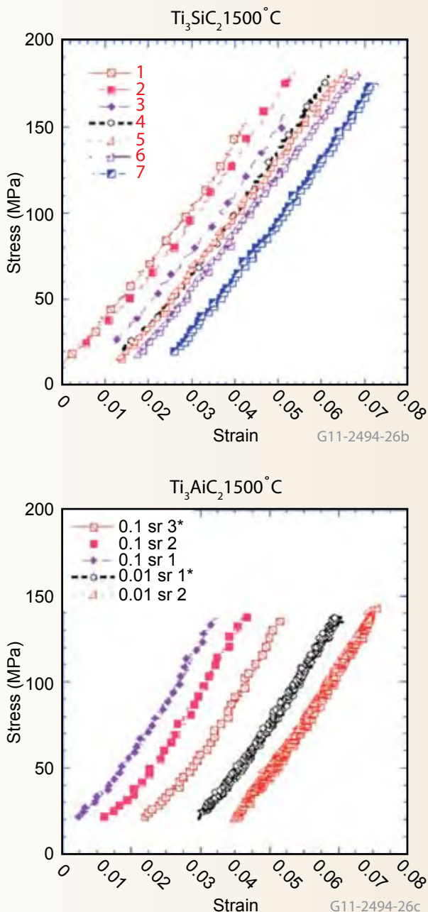
Figure 2. Engineering stress-strain curves for (a) \text{Ti}_3\text{SiC}_2 and (b) \text{Ti}_3\text{AlC}_2 . Each plot shows multiple test samples for each material.
