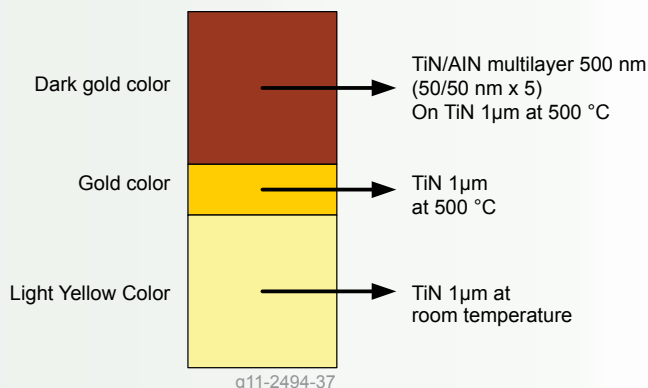
Figure 1. Schematic of TiN/AlN and TiN-coated large bars (HT-9 and MA957) for heavy ion irradiation test.
