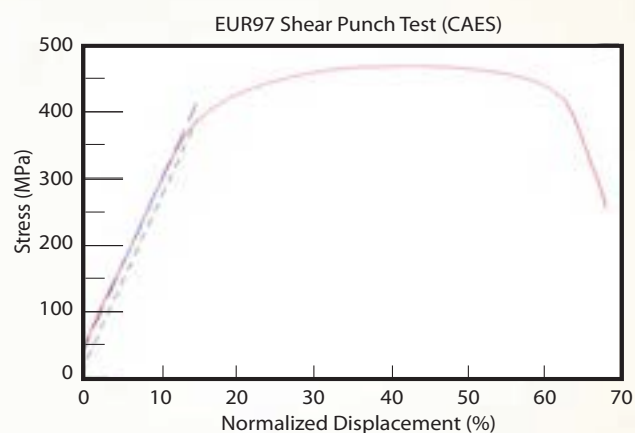
Figure 3. Load displacement data converted to engineering shear stress and strain.
