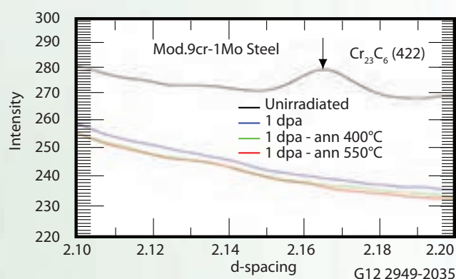
Figure 1. X-ray diffraction measurements of irradiated and irradiated-annealed mod.9Cr-1Mo steels showed the disappearance of Cr_{23}C_6 carbide diffraction peaks after irradiation to 1 dpa. Post-irradiation annealing showed no effect on the phase transformation.
