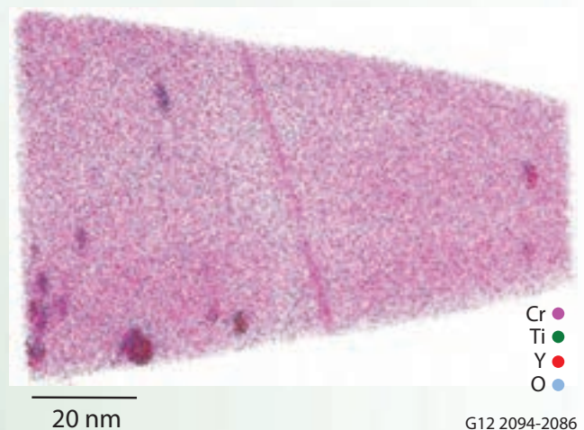
Figure 1. 3D reconstruction from an ODS steel showing Cr segregation at a grain boundary and the presence of oxide nanoparticles.
