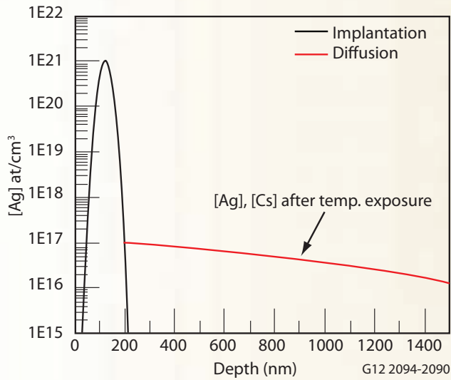
Figure 1. Schematic of ion implantation diffusion couple.
