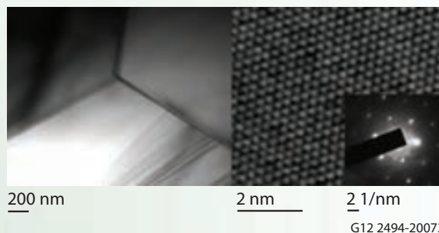
Figure 1. TEM micrographs of unirradiated \text{Ti}_3\text{AlC}_2 showing: a) a low-resolution, bright-field image of a triple point, b) a high-resolution image near the edge of the bottom grain in Figure 1(a). The inset shows a selected-area diffraction pattern from the same region with hexagonal symmetry of the basal planes.
