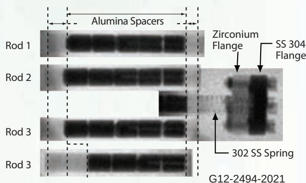
Figure 1. Neutron radiographs of four liquid metal gap filled fuel rod assemblies.
