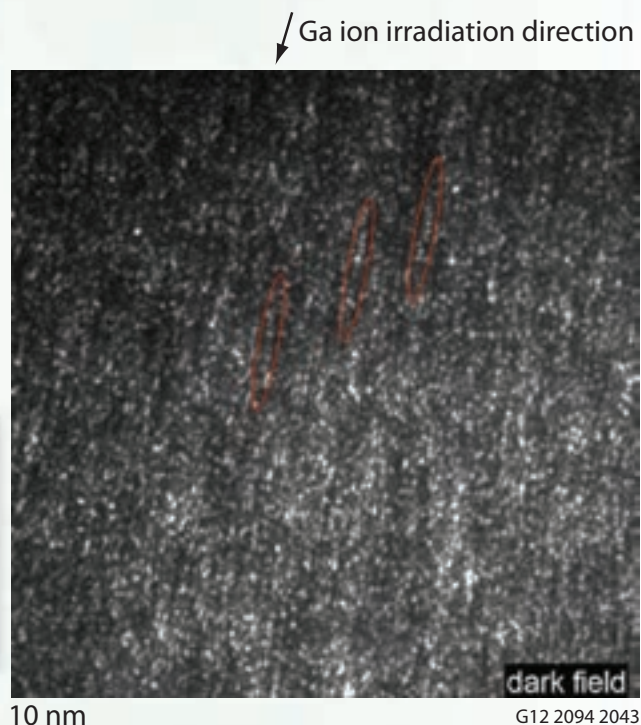
Figure 1. Dark-field TEM image of \text{Cu}_{50}\text{Zr}_{45}\text{Ti}_5 metallic glass specimen showing chained nanocrystals. This finding suggests that damage cascades can convert the metallic glass into nanometer-sized crystals.
