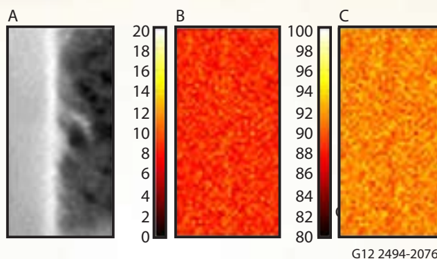
Figure 3. Annular dark-field image of lath boundary in as-received model steel, B) weight percent chromium map (bulk concentration: ~8.68% Cr), C) weight percent iron map.
