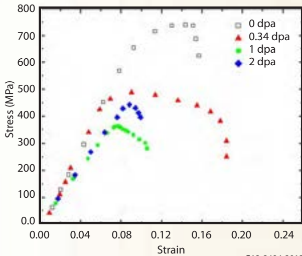
Figure 1. Stress-strain curves of irradiated nanostructured copper at different damage levels. In-reactor grain growth is dominant at 0.34 dpa in terms of decrease of strength and increased ductility while at 2 dpa, material response is suggested to be controlled by irradiation hardening.
