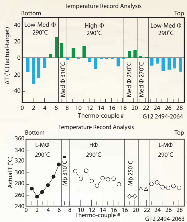
Figure 3. Actual temperature deviations from the calculated set points showing excellent overall thermal performance.
