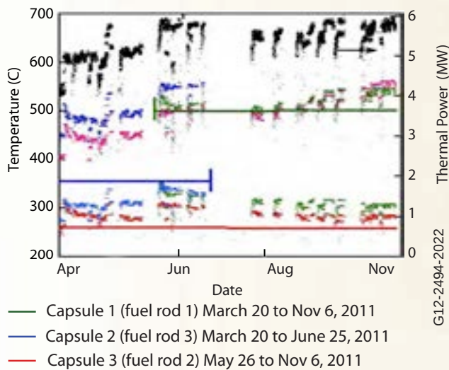
Figure 2. Center fuel rod and cladding temperature of fuel rods 1, 2 and 3 along with thermal power history.
