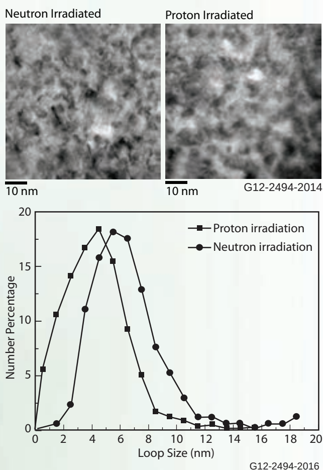
Figure 1. Comparison between ZrC neutron- and proton-irradiated to 1dpa at 800°C.
