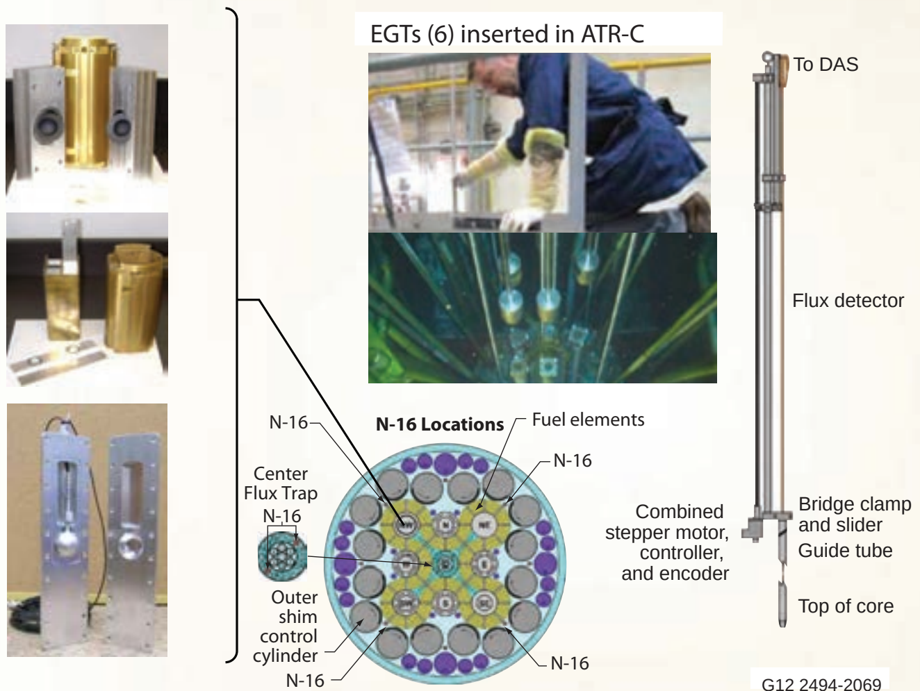
Figure 2. Specialized fixturing for flux detector evaluation in the NW-LIPT (left), and EGTs for evaluations in six N-16 positions (right).
