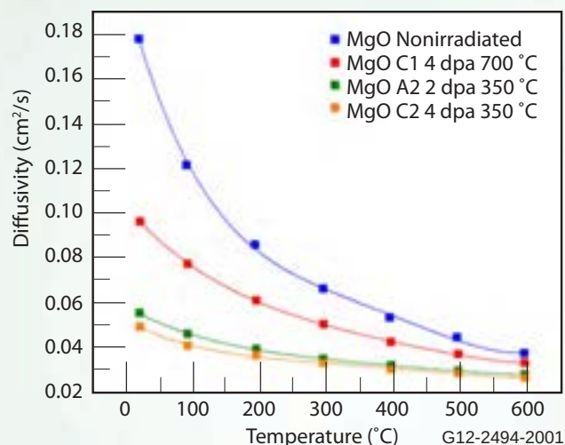
Figure 3. Thermal diffusivity of non-irradiated MgO compared to MgO irradiated under different conditions. Both MgO A2 and C2 show the most significant reductions in thermal diffusivity due to the high density of small dislocations, but there is little difference when the irradiation dose is increased. C1 irradiated at high temperature has an intermediate decrease in thermal diffusivity because of the lower density and larger size of the dislocations.
