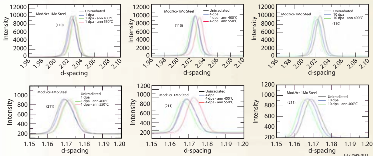
Figure 2. – Synchrotron XRD measurements of the irradiated and irradiated-annealed mod.9Cr-1Mo steel specimens showed peak shifts after irradiation and post irradiation annealing.
