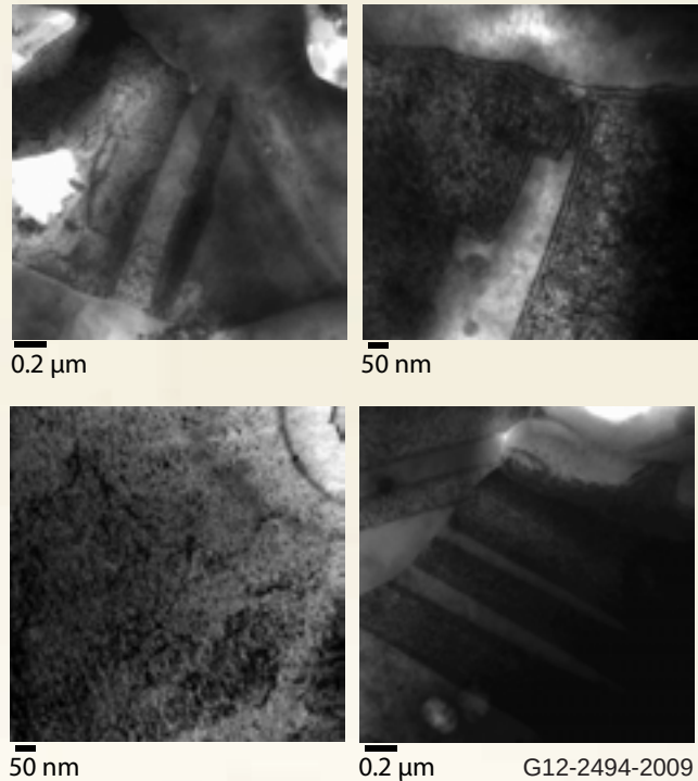
Figure 3. Annealing twins observed in nanostructured copper at 1 dpa (top left). Figure 4. Dislocation structures observed in nanostructured copper at 2 dpa (top right). Figure 5. Microstructure of irradiated micrograined copper showing the formation of dislocations causing radiation hardening (bottom left). Figure 6. Twin structure observed in micrograined copper (bottom right).
