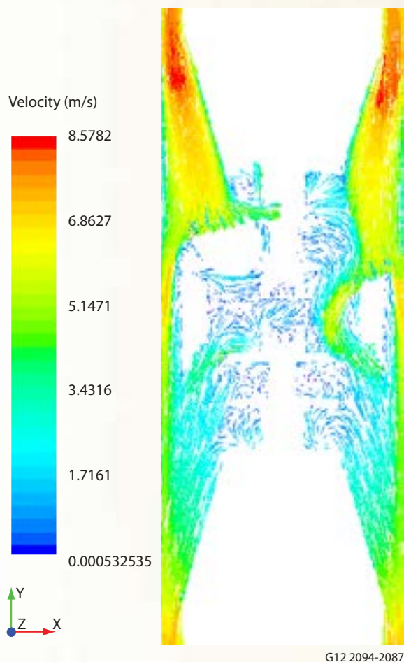
Figure 2. Velocity vectors in the z-normal plane of the hybrid capsule showing strong interactions between vortices that caused an increased pressure drop at a flow rate of 8 gpm.
