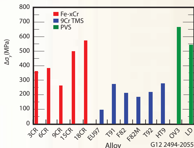
Figure 1. Examples of hardening in Fe-Cr binary alloys (red), 9Cr tempered martensitic steels (blue) and a model RPV alloy and steel (green).
