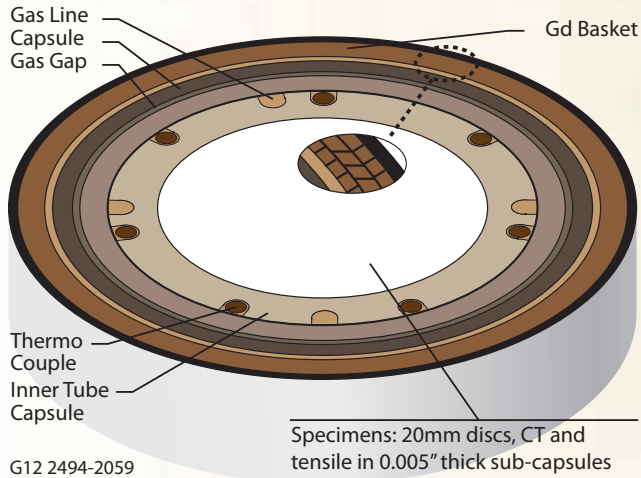
Figure 1. Cross section of the UCSB ATR-2 test assembly.
