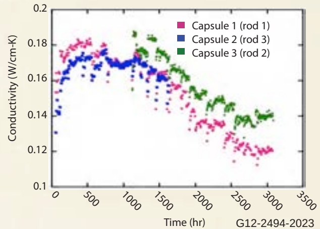
Figure 3. Thermal conductivity variation with irradiation exposure for thermal power greater than 4 MW.
