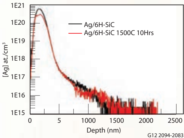
Figure 2. SIMS depth profiles of Ag in 6H-SiC, as implanted at 1500°C under 10 hours of exposure.
