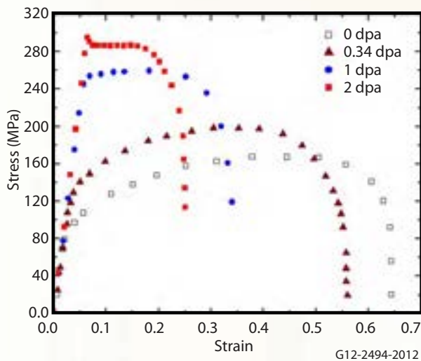
Figure 2. Stress-strain curves of irradiated micrograined copper showing irradiation hardening at all damage levels.
