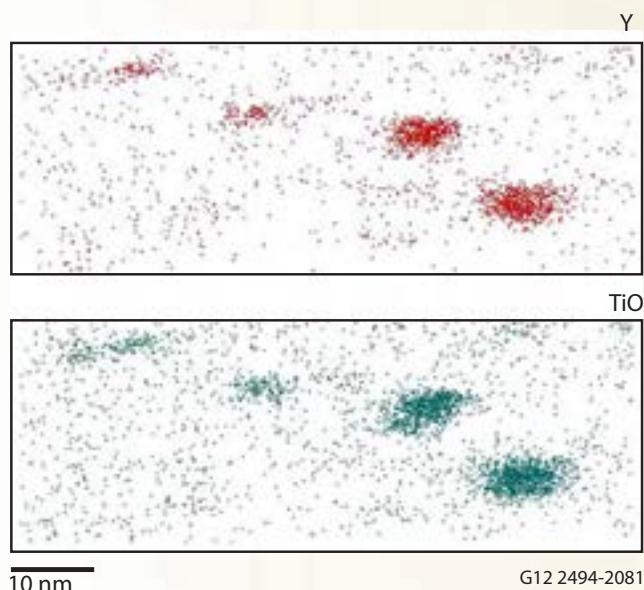
Figure 1. APT atom maps of the as-received (unirradiated) 9%CrODS showing nanoclusters of (Y, Ti) oxide.
