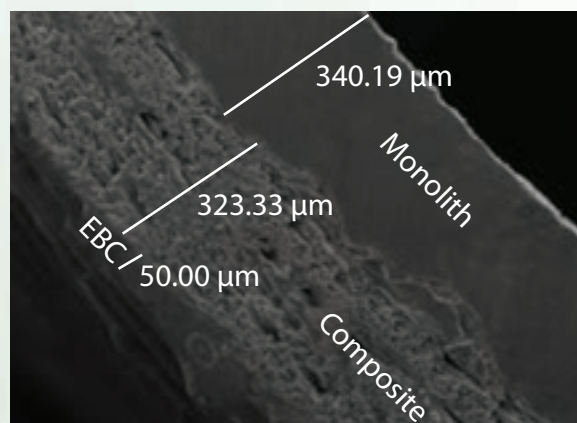
Figure 1. SEM micrograph cross section showing the three layers of the triplex cladding design.
