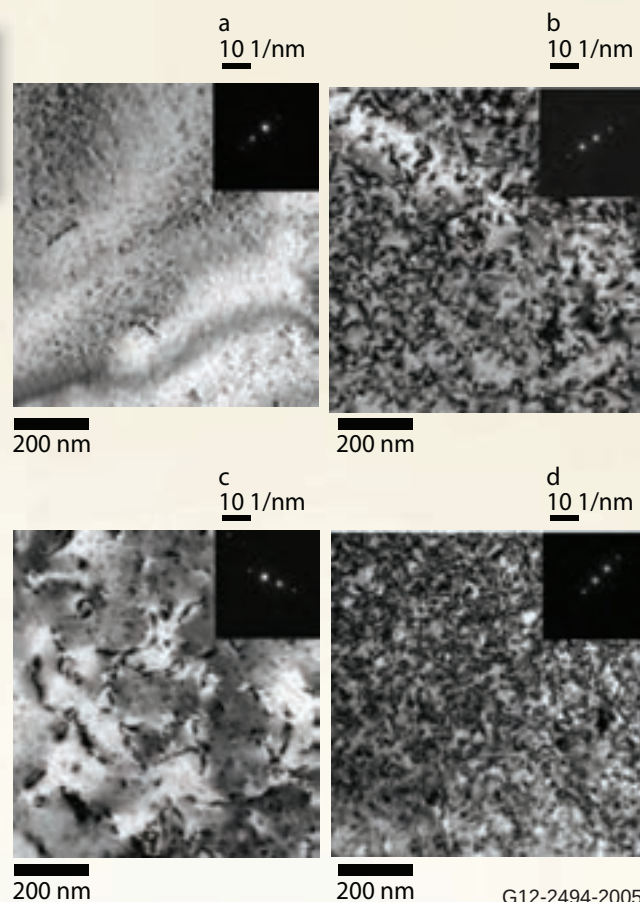
Figure 2. Results of MgO TEM. Figure 2a: Minimal ion damage due to the FIB in non-irradiated MgO. Figure 2b: High-density TEM of small dislocation loops due to neutron irradiation in A2 MgO. Figure 2c: C1 MgO has a lower density of larger dislocations due to the higher irradiation temperature. Figure 2d: C2 MgO has a higher density of dislocations compared to A2 MgO because of the larger irradiation dose. Each TEM image is in the g = [200] two-beam diffraction condition.
