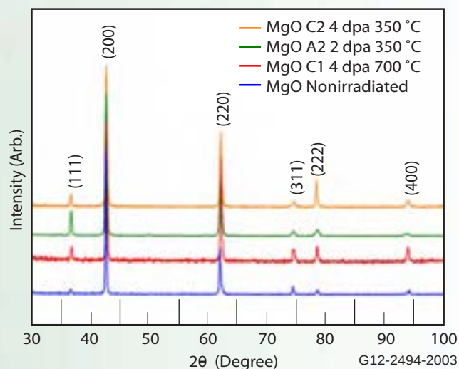
Figure 1. XRD of \text{MgO} indicates the material did not become amorphous after irradiation and the crystal structure did not change.
