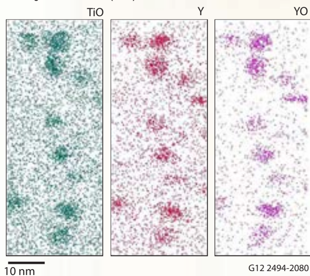
Figure 2. APT atom maps of the 9%Cr ODS sample neutron-irradiated to 3 dpa at 500°C, indicating the stability of (Y, Ti) oxide nanoclusters after irradiation. Samples of 9%Cr commercial ferritic steel NF616 irradiated at the ATR NSUF at 500°C to a level of 3 dpa were characterized using scanning transmission electron microscopy (STEM) and APT.
