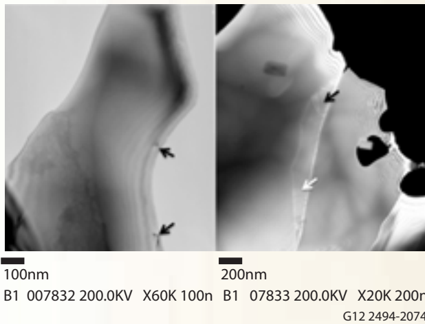
Figure 2. TEM micrographs of \text{Ti}_3\text{SiC}_2 irradiated with a Cf neutron source to a dose of \sim 10^{-7} dpa. As expected, such a low dose resulted in no visible irradiation damage. Dislocations (black arrows) and stacking faults (white arrow) can be seen in both the a) bright-field and b) dark-field images of different regions.
