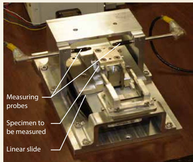
Figure 4. Remote precision measurement device designed and built by INL.
