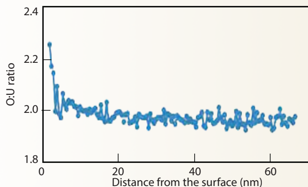
Figure 2. O:U ratio measured by APT of a surface from single-crystal \text{UO}_2 indicating hyperstoichiometry at the surface.
