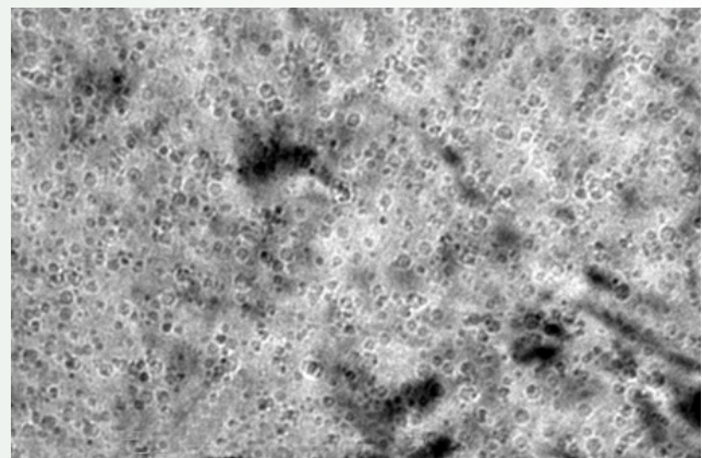
Figure 6. TEM images showing higher density of smaller cavities/bubbles in cooler region.
