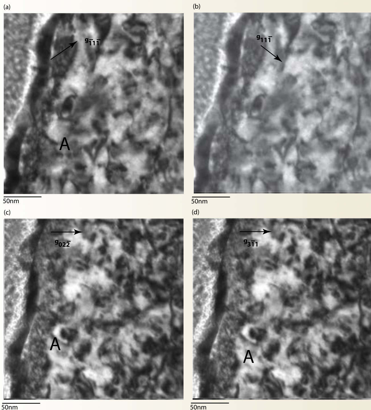
Figure 2. Series of TEM images used for part of the dislocation loop analysis in the \text{UO}_2 single crystal irradiated with 1-MeV Kr ions at 800° C to a dose of 5 \times 10^{15} ions/cm 2 . The arrows denote the direction of g : (a) g = [\bar{1}1\bar{1}] ; (b) g = [11\bar{1}] ; (c) g = [02\bar{2}] ; and (d) g = [3\bar{1}1] . In each analysis, the beam direction is close to [001] .
