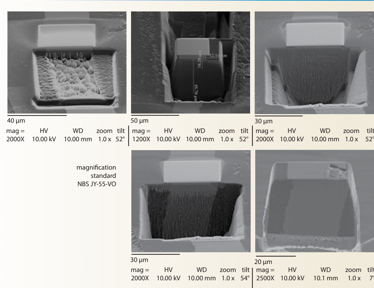
Figure 2. Examples of FIB milling techniques of a TRISO SiC layer annealed at 1600° C for one hour (sample batch B).
