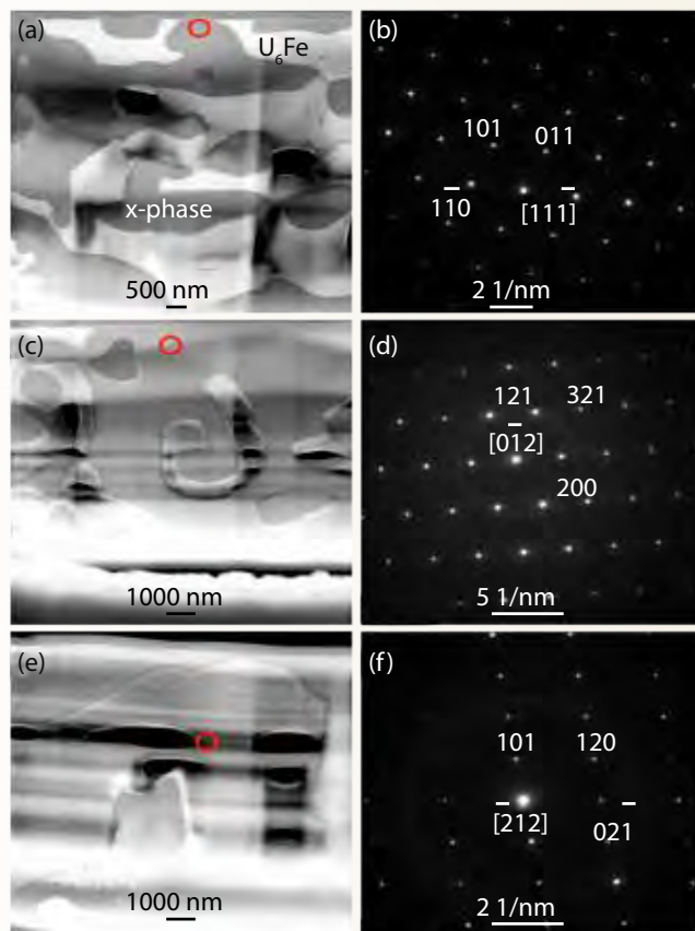
Figure 2. The complex ternary phases, \text{Fe}(\text{Zr,U})-\chi (oP8), \text{Fe}(\text{Zr,U})_2-\epsilon (tI12) and \text{U}_3(\text{Zr,Fe})-\lambda (tI12) phases developed in the U-10wt.% Zr versus Fe diffusion couple annealed at 953K. TEM analysis via sample preparation with FIB in-situ lift-out (INLO) has identified their crystal structures for the first time.
