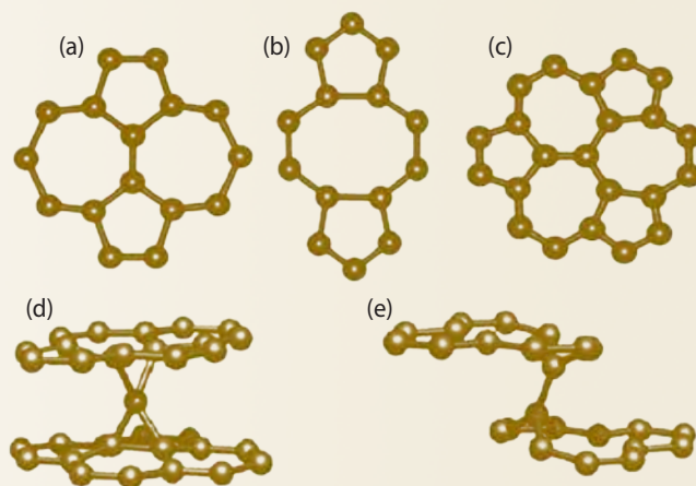
Figure 2. (a, b, c): Three topological defect configurations: Stone-Wales 55–77, 5–8–5, and 555–777; (d, e): delineations of two interplanar defect configurations: spiro and divacancy.*
