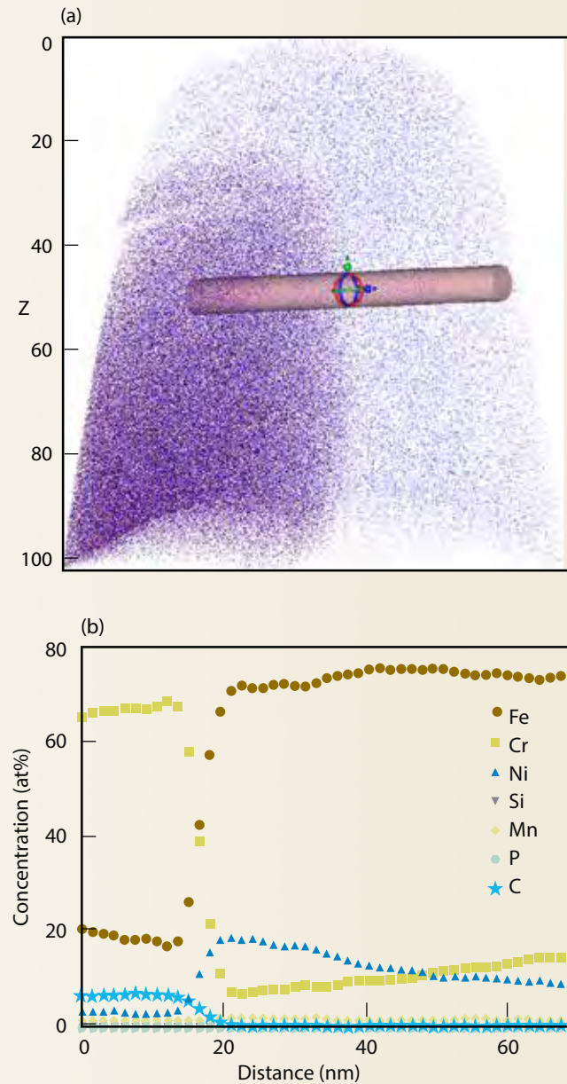
Figure 4. (a) Atom probe reconstruction of a 40^\circ [8\ 9\ 4] , carbide-grain boundary interface in 304SS, irradiated in the EBR-II to 4.5 \times 10^{21} \text{ n/cm}^2 . (b) Corresponding concentration profile of an interface highlighting Cr-rich carbide and adjacent Cr-depleted region.
