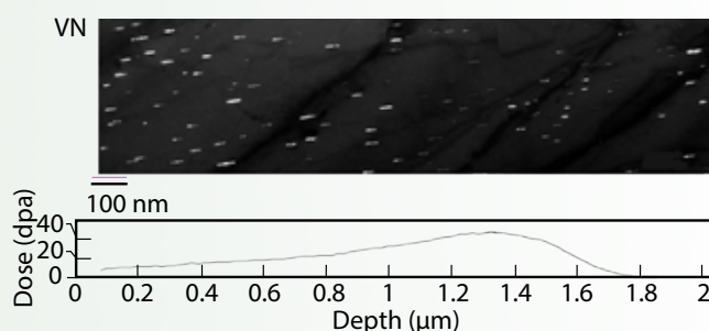
Figure 1. Dark field image showing the evolution of VN precipitates (white) under \text{Fe}^{2+} irradiation at 500^\circ\text{C} starting from the irradiated surface (left) to bulk matrix without irradiation (right). The dose increases are shown in the Stopping and Range of Ions in Matter (SRIM) simulated depth-dependent irradiation dose profile beneath the image.
