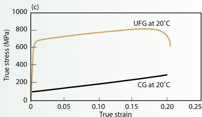
Figure 1. (a) TEM micrograph of UFG Fe-14Cr-16Ni. (b) Chart showing the average grain size in the samples is \sim 400\text{ nm} . (c) Graph showing the yield strength has increased from 100 megapascals (MPa) for a CG sample to over 600 MPa for a UFC sample with good ductility.
