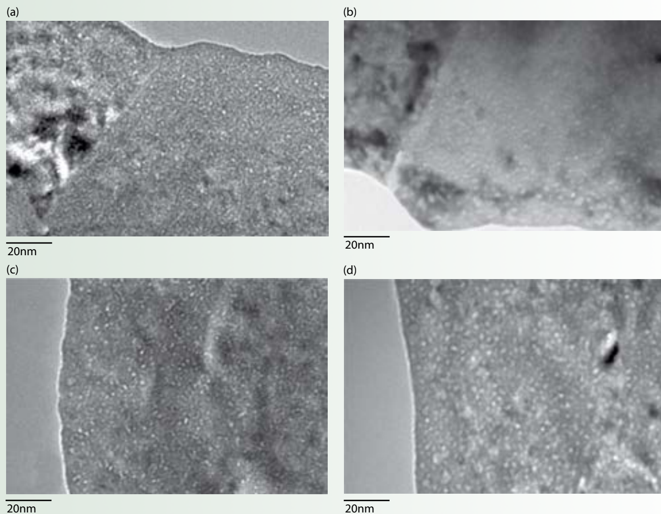
Figure 3. TEM images showing bubbles in UO 2 irradiated up to a final dose of 5 \times 10^{15} ions/cm 2 with 150-keV Kr at (a) 25° C and (c) 600° C, and (b and d) 1-MeV Kr at 800° C. (a) and (b) are polycrystalline UO 2 ; (c) and (d) are single-crystal UO 2 .
