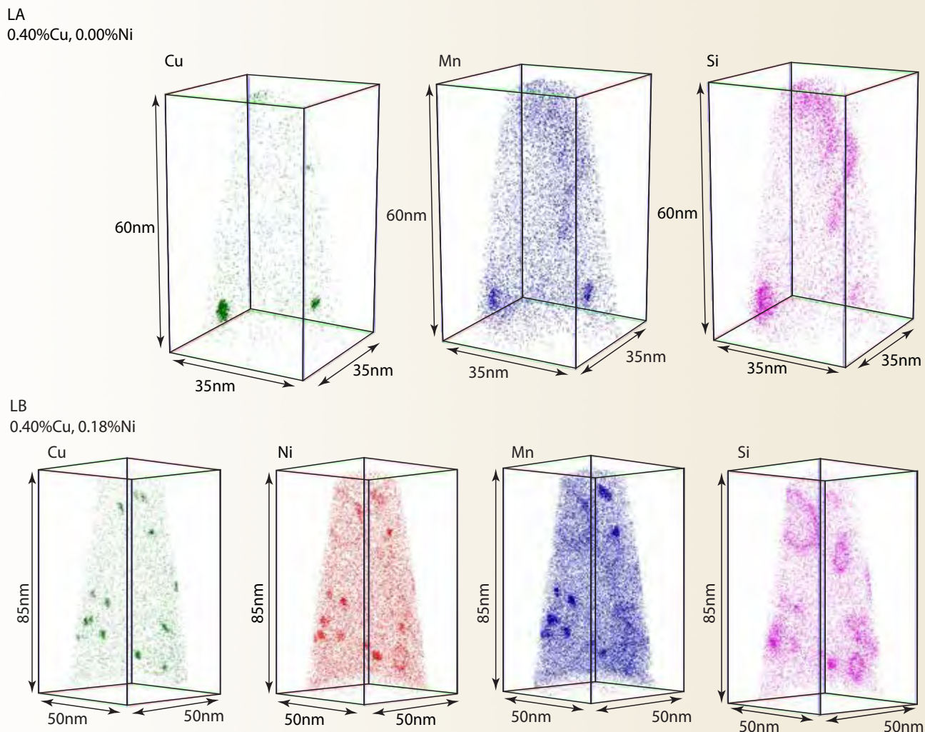
Figure 1. Atom maps of two high-Cu steels. Top is a Ni-free alloy (LA) and bottom is a low, 0.18wt.%Ni (LB) alloy. The Ni-free steel contains fairly large, coarse precipitates that have a Cu-rich core surrounded by a Mn- and Si-rich “cloud.” The low-Ni steel contains a higher density of smaller Cu-Ni-Mn-Si clusters.
