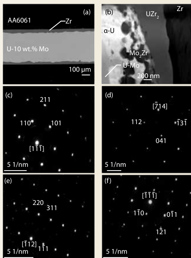
Figure 3. (a) and (b) Typical backscatter electron micrograph of the U-10wt.%Mo monolithic fuel interaction with the Zr diffusion barrier, with reaction kinetics (e.g., thickness). (c-f) Phase identification by TEM analysis via sample preparation with FIB-INLO. Selected area electron diffraction patterns from (c) \gamma -U(Mo) solid solution, (d) \alpha -U, (e) \text{Mo}_2\text{Zr} , and (f) \text{UZr}_2 phases at the interface between U-10wt.%Mo monolithic fuel and the Zr diffusion barrier.
