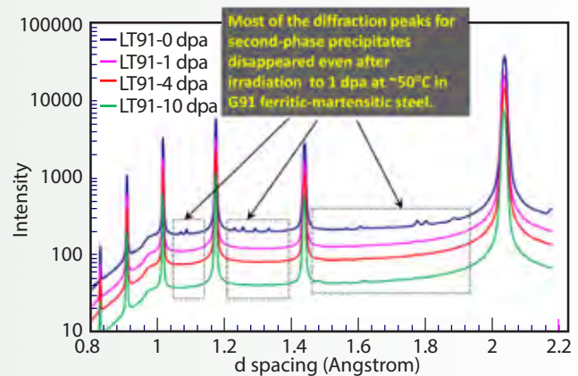
Figure 1. Diffraction peaks in irradiated G91.
