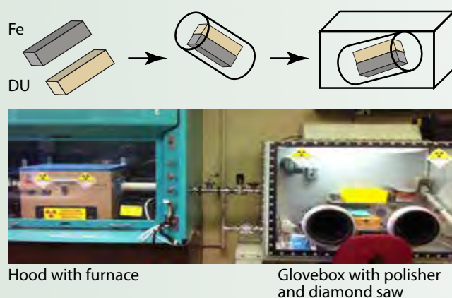
Figure 1. Fabrication of uranium-bearing diffusion couples at TAMU.
