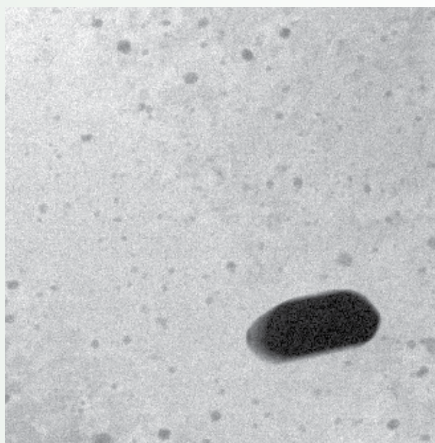
Figure 1. TEM image of the parent MA956 alloy irradiated to 1 dpa.
