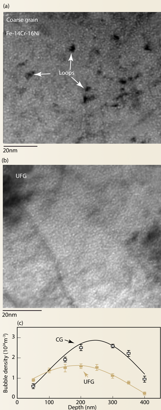
Figure 2. TEM micrograph of He ion irradiated Fe-Cr-Ni alloy ( 100\text{ keV}/6 \times 10^{16}/\text{cm}^2 at peak damage ( \sim 5 displacements per atom [dpa])). (a) CG alloys have a high density of He bubbles and dislocation loops. (b) In the UFG alloy, no dislocation loops were observed. (c) Graph showing He bubble density in the UFG alloy was two times lower than that of the CG alloys.
