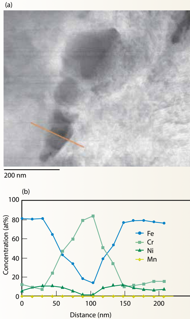
Figure 3. (a) STEM image illustrating M23C6 Chromium (Cr)-rich carbides along a 49^\circ [2\ 3\ 9] grain boundary. (b) Corresponding STEM-EDS line profile from Cr-rich carbide.
