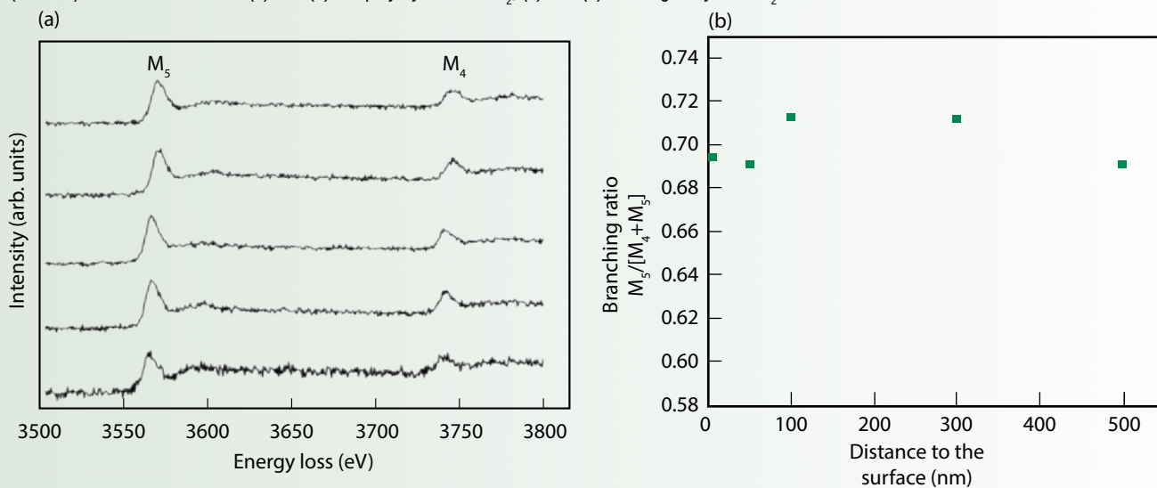
Figure 4. (a) EELS spectra as a function of the distance to the surface showing the M 4 and M 5 edges of U in 1 MeV Kr-irradiated UO 2 up to a dose of 5 \times 10^{15} ions/cm 2 and (b) the branching ratio, M_5/(M_4 + M_5) , profile as a function of the distance to the surface.
