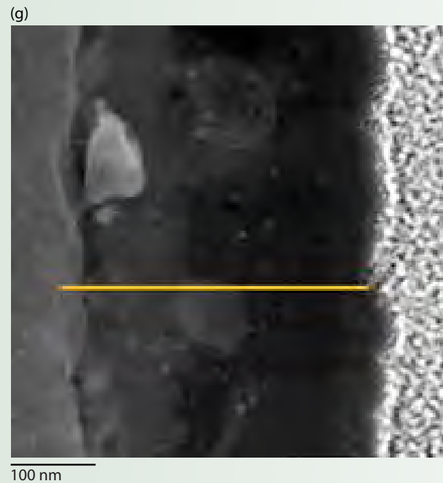
(g and h) irradiated \text{Y}_2\text{O}_3 samples. Horizontal lines in the images represent the EDS line-scan distances in the interface regions (the region on the left side of the images is the substrate).
