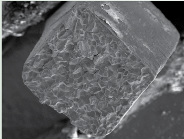
200 μm SE Overview 100x
