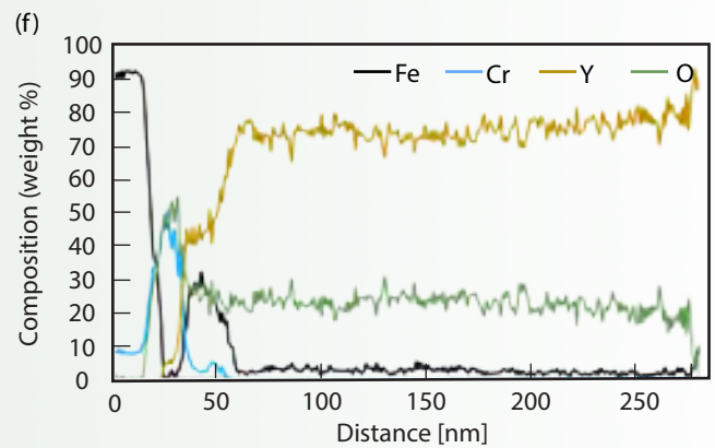
Figure 1. (cont.) STEM images and EDS elemental line scans of the \text{TiO}_2 (e and f) thermally exposed \text{Y}_2\text{O}_3 -coated samples; and
