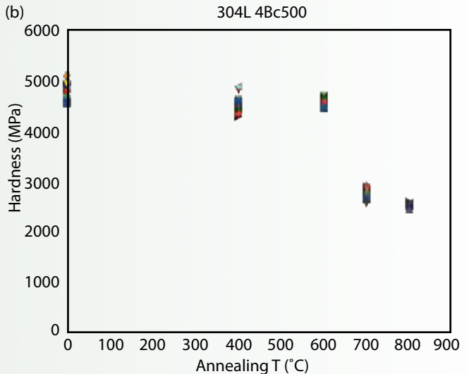
Figure 3. (a) TEM micrograph of the equal channel angular processed NC 304L SS sample. The average grain size is ~100 nm by 250 nm. (b) Graph showing the hardness of the sample remained the same after annealing up to 600° C/10h.
