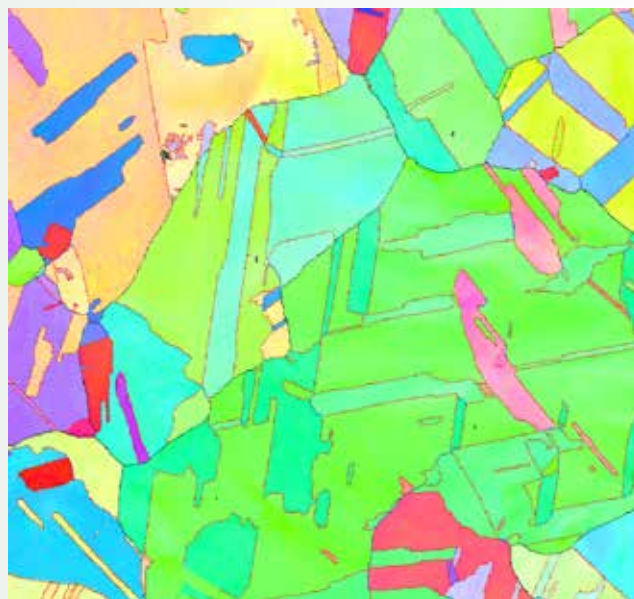
Figure 1. SEM-EBSD inverse-pole image highlighting the grain boundary character distribution in the 304SS sample (U1302), which indicates high densities of \Sigma 3 , \Sigma 9 , and random high-angle grain boundaries.
