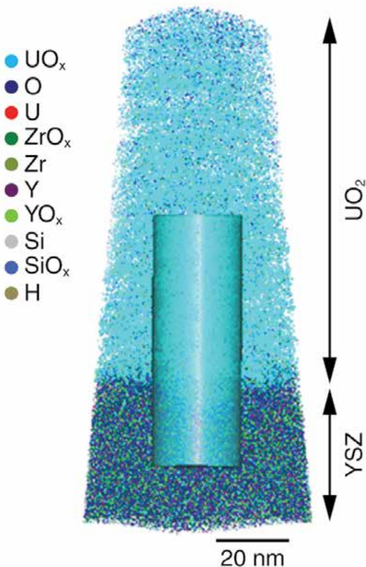
Figure 1. 3D APT reconstruction of the elements in the UO 2 /YSZ thin film. Complex ions represented as UO x , ZrO x , YO x , where x = 1, 2 , or 3 .
