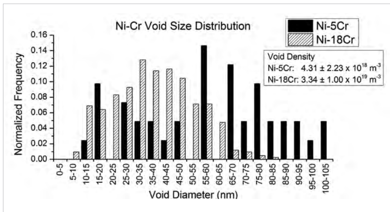
Figure 2. Void density and size distribution in 500°C proton-irradiated Ni-Cr.
