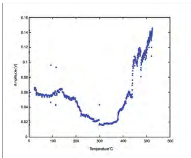
Figure 4. Temperature-dependent performance of an AlN piezoelectric transducer. The transducers operated at their highest efficiencies at the design temperature.
