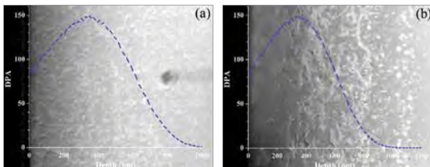
Figure 5. (a) Cross-section STEM images showing the dislocations in as-irradiated and annealed polycrystalline \text{UO}_2 at 1300^\circ\text{C} for one hour. (b) Dashed lines show the damage profiles in displacements per atom (dpa) calculated by stopping-and-range-of-matter-in-ions (SRIM) software.
