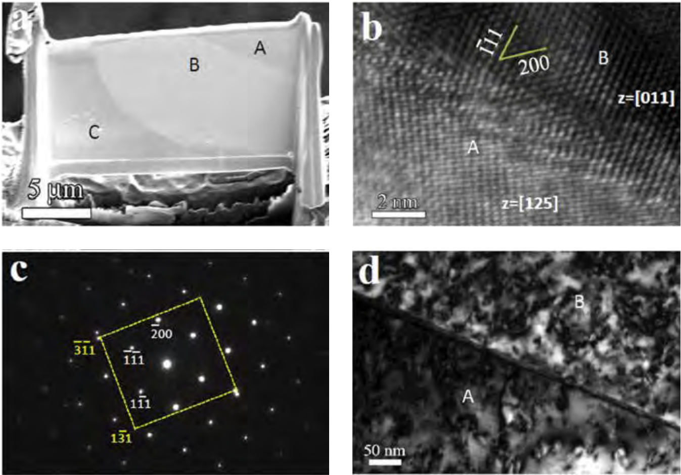
Figure 4. (a) A scanning electron microscope (SEM) image of a TEM lamina prepared by FIB showing three grains, A, B, and C. (b) High-resolution TEM image showing the grain boundary between grains A and B, the orientations of grains A and B are close to [125] and [011], respectively. (c) Selected-area diffraction pattern of grains A and B. (d) Bright-field TEM images showing the dislocation loops in grains A and B that have been irradiated with 1 MeV Kr at 600°C at a dose of 5 \times 10^{14} ions/cm 2 .
