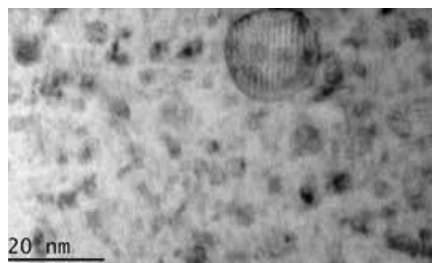
Figure 1. A TEM image of the oxide particles observed in the 14LMT alloy specimen unirradiated at 500°C.
