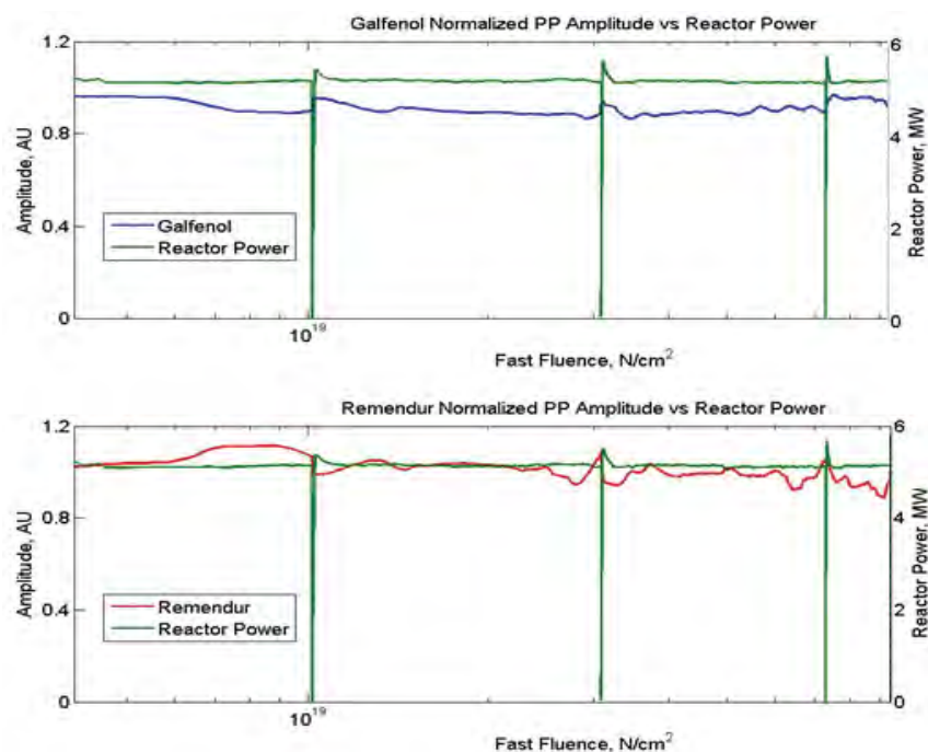
Figure 9. Pulse-echo amplitude of the Galfenol and Remendur magnetostrictive transducers.
