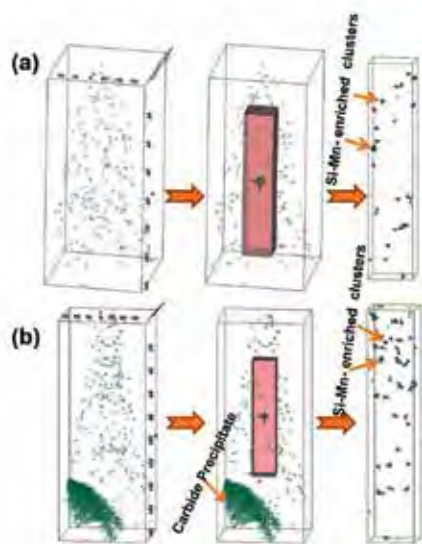
Figure 3. Si-Mn-enriched cluster distribution post-neutron irradiation for (a) CG and (b) UFG steel. The dimension of the interior (colored) boxes is 20 x 20 x 100 nm.
