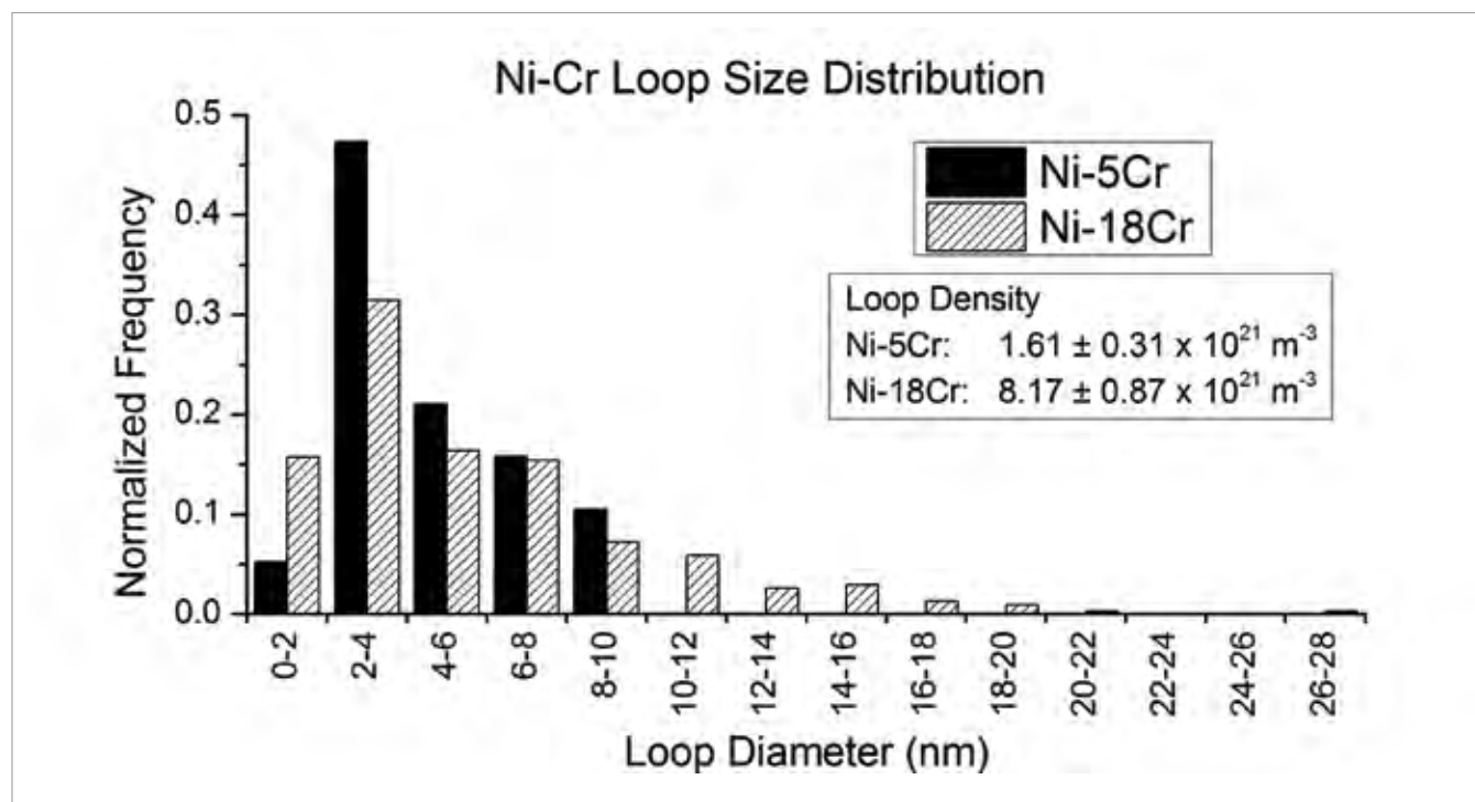
Figure 1. Dislocation loop density and size distribution in 500°C proton-irradiated Ni-Cr.
