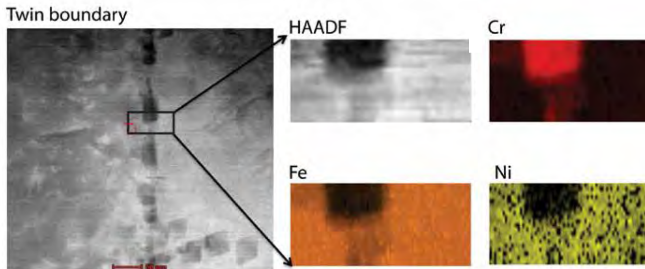
Figure 1. STEM and STEM-EDS results from a twin \Sigma 3 grain boundary highlighting characteristic Cr rich M_{23}C_6 carbides along the examined GB length.
