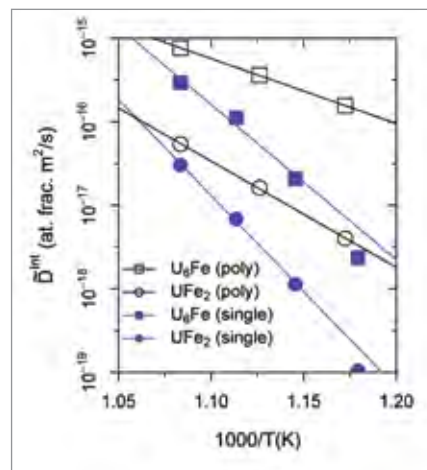
Figure 1. Comparisons of integrated diffusivities forming UFe_2 and U_6Fe phases in U-Fe diffusion couples using polycrystalline Fe and single crystal Fe, respectively.
