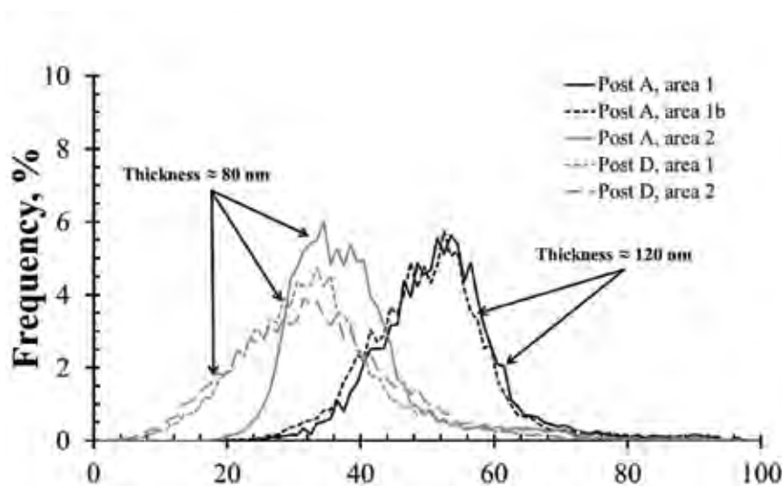
Figure 3. Frequency distribution of the Index parameter showing thicker samples yield higher quality orientation data.
