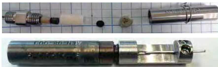
Figure 2. Piezoelectric transducer fabrication. (Top) Transducer components from left to right: stainless steel cap, alumina insulation, nickel plunger, alumina insulation, carbon-carbon backing, Kovar waveguide with ZnO sensor on top, stainless steel outer casing. (Bottom) A fully assembled transducer housing with cable and strain-relief sleeve to support the cable connection.
