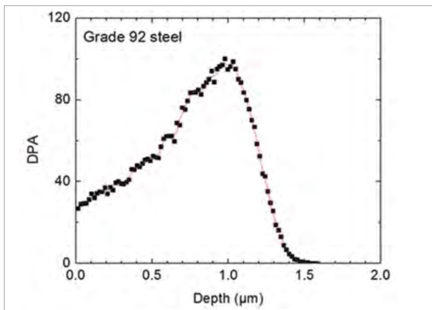
Figure 1. The calculated irradiation damage profile in terms of dpa versus length.
