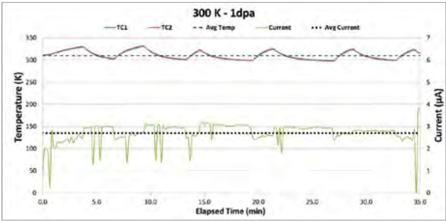
Figure 6. Temperature and beam-current profiles during irradiation at 300 K, 1 dpa, and 2.0 MeV C + .
