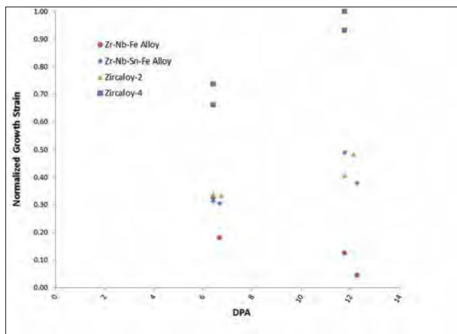
Figure 1. Measured growth strain of selected Zr alloys as a function of dpa, normalized using the maximum growth strain.
