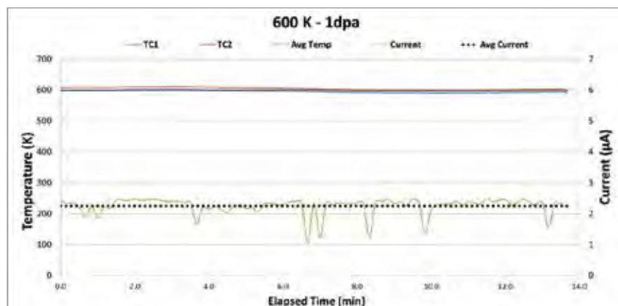
Figure 5. Temperature and beam-current profiles during irradiation at 600 K, 1 dpa, and 2.0 MeV C^+ .
