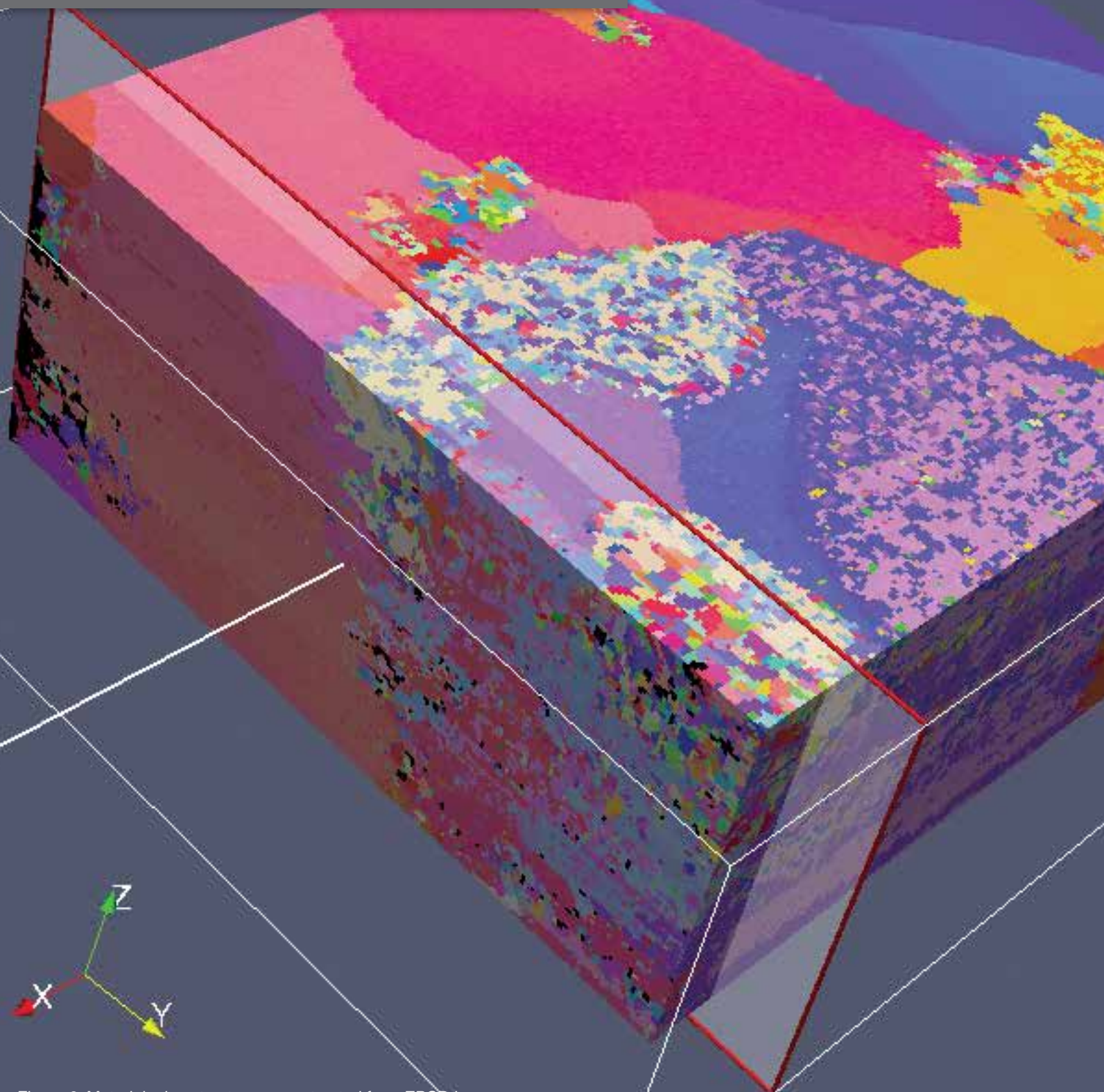
Figure 2. Material microstructure reconstructed from EBSD images.
