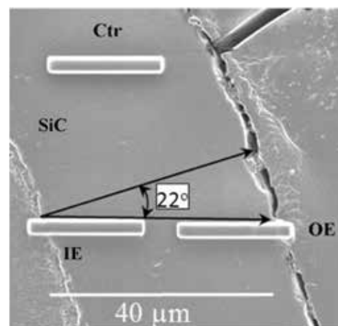
Figure 4. FIB lamellae positions on the SiC layer of sample AGR1-632-035.
