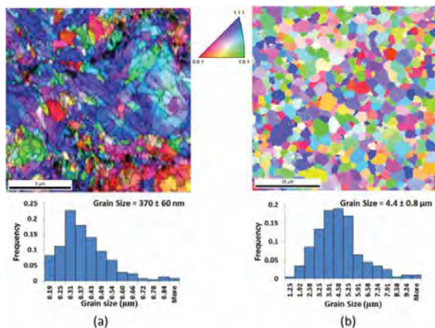
Figure 1. Pre-irradiation EBSD patterns and grain size distributions for (a) UFG and (b) CG steels.
