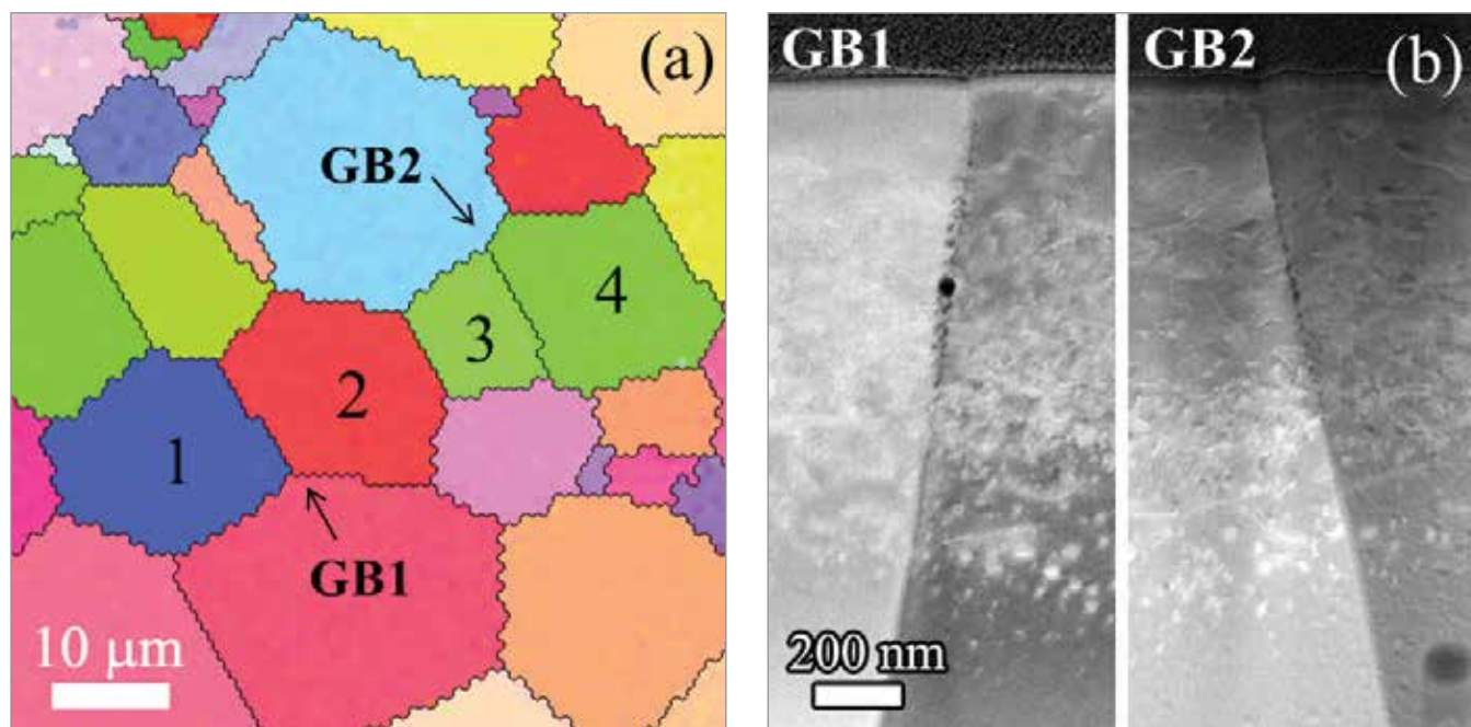
Figure 4. (a) Electronic backscatter diffraction (EBSD) map of Kr-irradiated, polycrystalline \text{UO}_2 annealed at 1300°C for one hour. Arrows mark a high-angle grain boundary between Grain 1 and Grain 2 (GB1) and a low-angle grain boundary between Grain 3 and Grain 4 (GB2). (b) Cross-section STEM images comparing the bubble distribution at GB1 and GB2.
