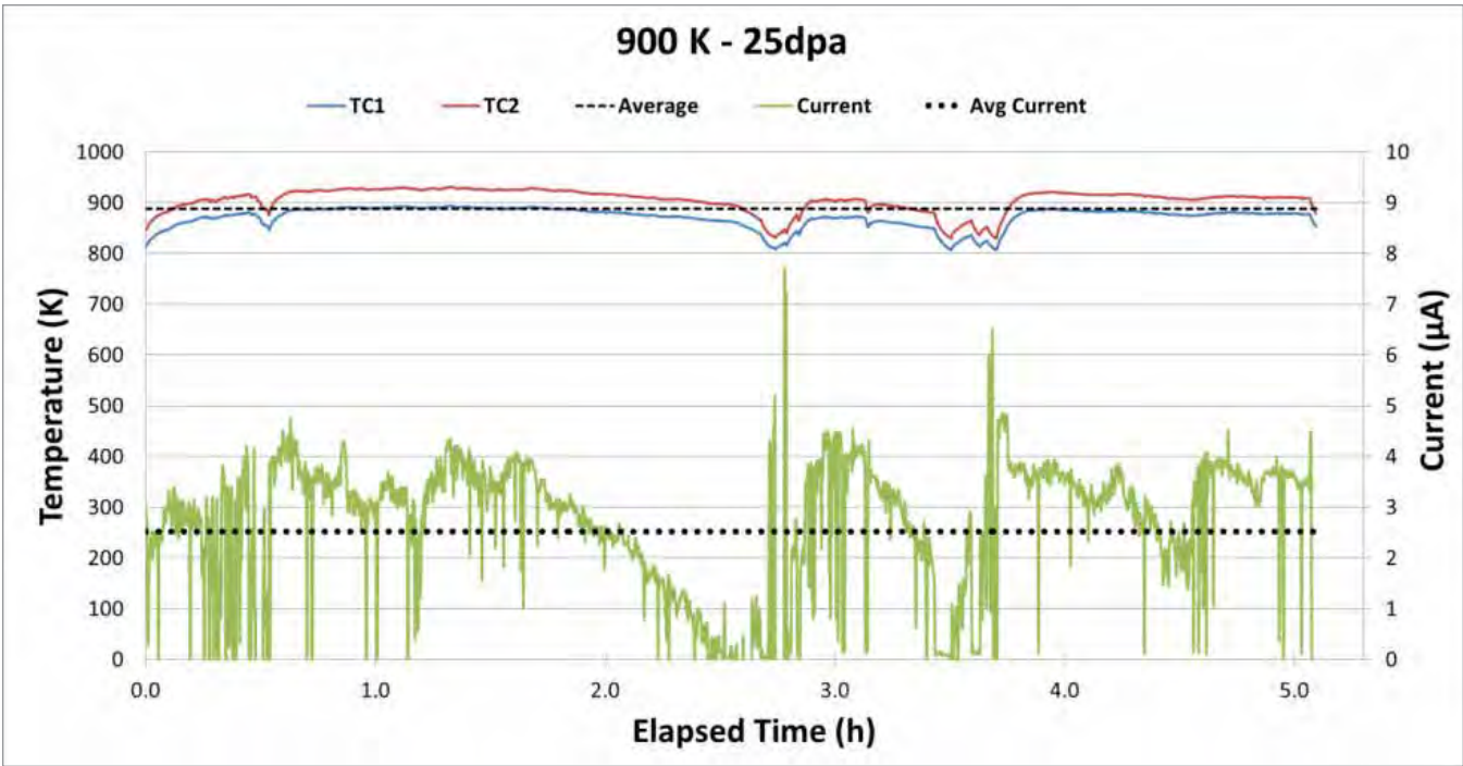
Figure 2. Temperature and beam-current profiles during irradiation at 900 K, 25 dpa, and 2.0 MeV C + .
