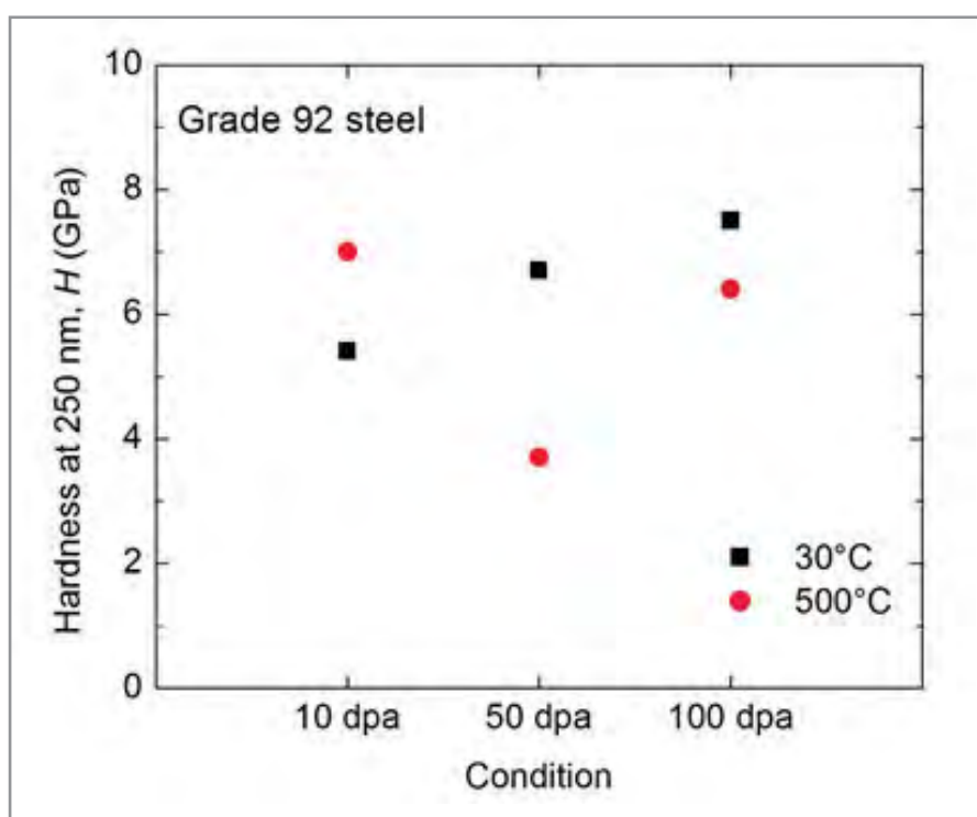
Figure 4. Hardness of Grade 92 steel as a function of irradiation dose at 30°C and 500°C.
