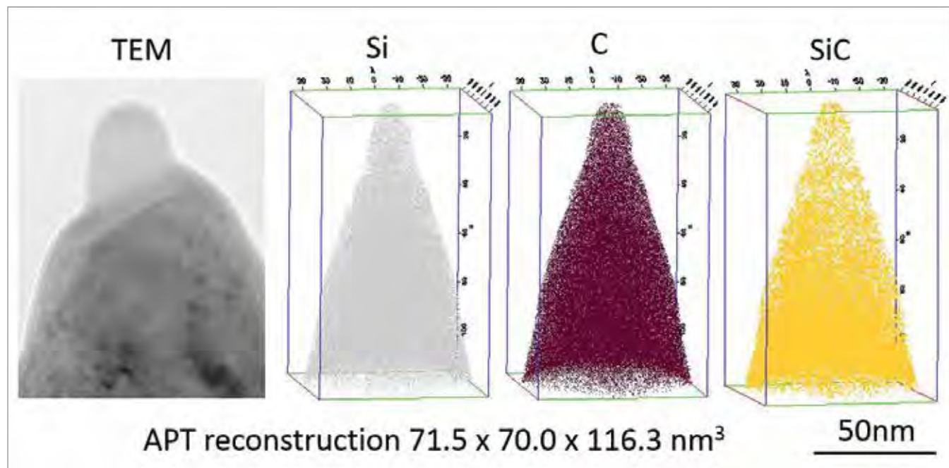
Figure 2. LEAP results showing the distribution of elements in a tip fabricated from a neutron-irradiated TRISO fuel particle.
