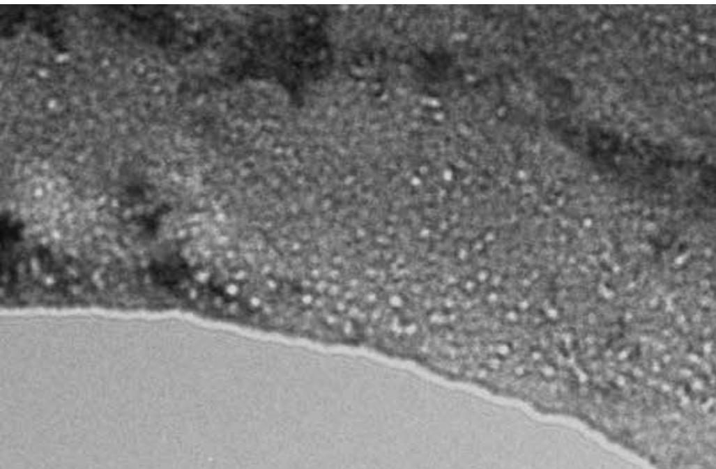
Figure 1. TEM images of bubbles in a \text{UO}_2 crystal implanted with Xe at a dose of 5 \times 10^{14} ions/ \text{cm}^2 .
