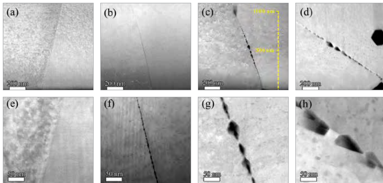
Figure 3. Cross-section scanning transmission electron microscope (STEM) images showing the evolution of intergranular bubbles during post-irradiation annealing at (a and e) 25°C, (b and f) 1000°C, (c and g) 1300°C, and (d and h) 1600°C. Figures (a-d) are low-magnification images, and figures (e-h) are high-magnification images. The dashed line in (c) indicates the bubbles' distance from the sample's surface.
