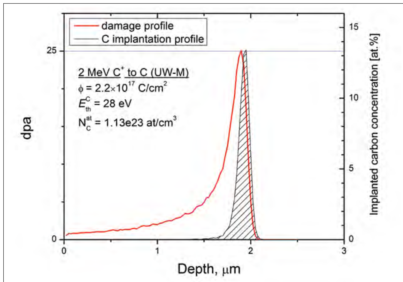
Figure 1. MeV carbon-implantation and damage profiles calculated using SRIM 2012.03 software.
