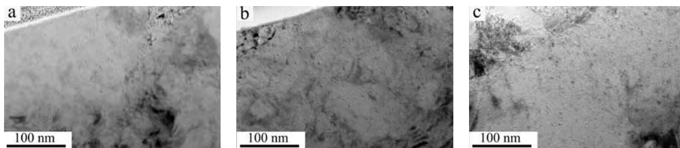
Figure 3. TEM images of irradiated Grade 92 specimens under two-beam bright field conditions at a) 10 dpa/30°C, b) 50 dpa/500°C, and c) 100 dpa/500°C.
