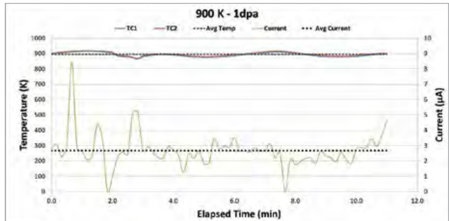
Figure 3. Temperature and beam-current profiles during irradiation at 900 K, 1 dpa, and 2.0 MeV C^+ .
