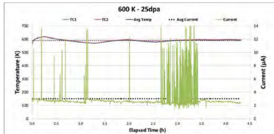
Figure 4. Temperature and beam-current profiles during irradiation at 600 K, 25 dpa, and 2.0 MeV C^+ .
