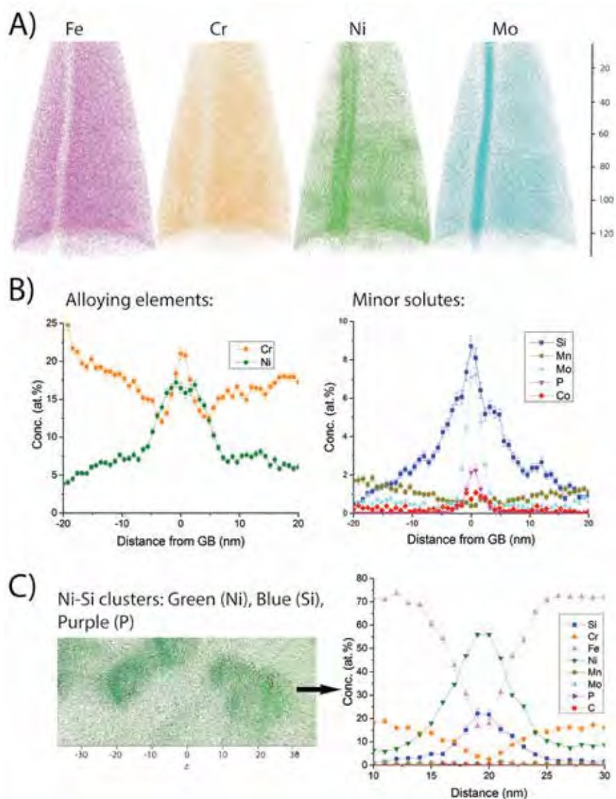
Figure 4. (A) Sequence of atom probe tomography atom map for Fe, Cr, Ni, Mo, (B) highlighted GB microchemistry including Cr depletion with "W" profile, and (C) concentration profile for Ni-Si enriched clusters.
