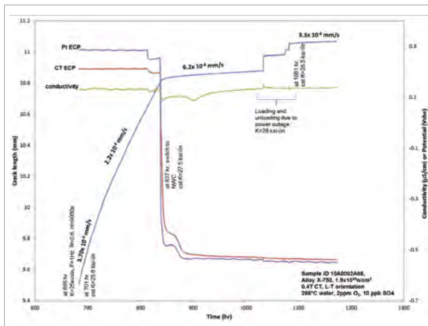
Figure 5. IASCC test results for X-750 irradiated to 1.93 \times 10^{20} n/cm 2 . CGR is the dark blue line.
