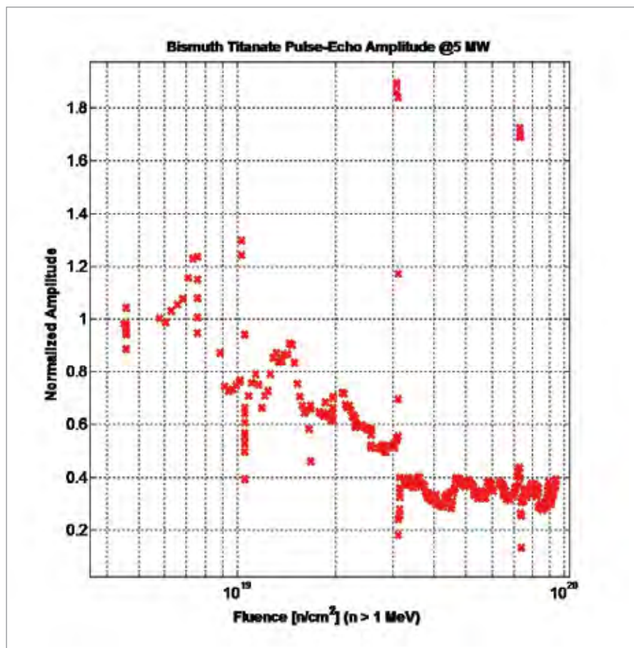
Figure 8. Pulse-echo amplitude measured for the BiT transducer during the first power cycle.
