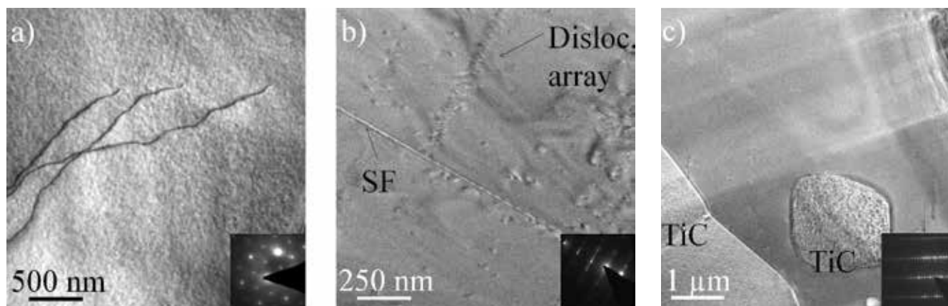
Figure 1. a) Brightfield TEM images taken near the (0001) zone axis of the ATR- \text{Ti}_3\text{SiC}_2 sample irradiated to 0.1 dpa at 100°C reveals perturbation of the surface and long basal plane dislocations. The mottled surface was likely due to improper FIB cleaning. b) TEM micrograph of ATR- \text{Ti}_3\text{SiC}_2 sample irradiated to 0.1 dpa at 500°C taken in 2 beam condition near the (11-20) zone axis shows dislocation arrays parallel to the basal plane and stacking faults. Small defects can be seen throughout, but were not confirmed as loops. c) Brightfield TEM micrograph taken on the (11-20) zone of the ATR- \text{Ti}_3\text{SiC}_2 sample irradiated to 0.1 dpa at 1000°C showing a preexisting TiC particle that was highly damaged - with dislocation loops and black spots - not present in the surrounding MAX matrix, which remains clear of irradiation induced defects.
