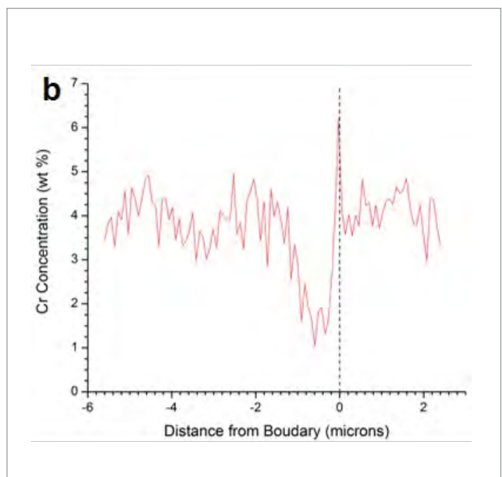
Figure 3. Typical RIS profile observed in 500°C proton-irradiated materials. A large Cr-depleted region is observed that is also denuded in voids and dislocations.
