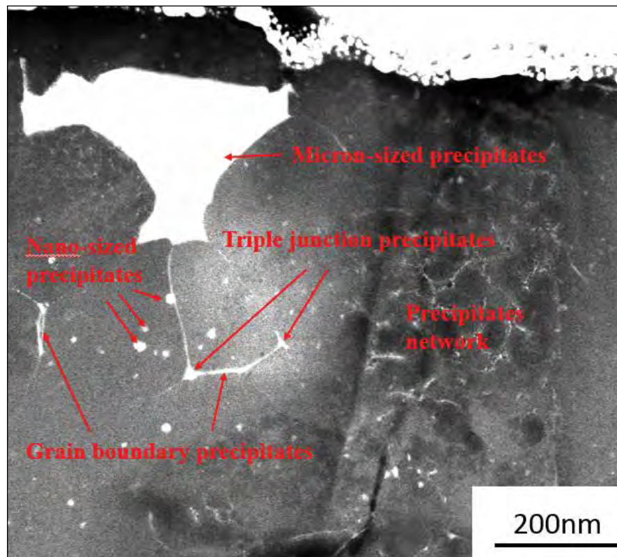
Figure 1. Distribution of FP precipitates in the SiC layer (~5 \mu\text{m} from SiC/IPOyC interface) of a neutron-irradiated TRISO fuel particle from AGR-1 experiments.
