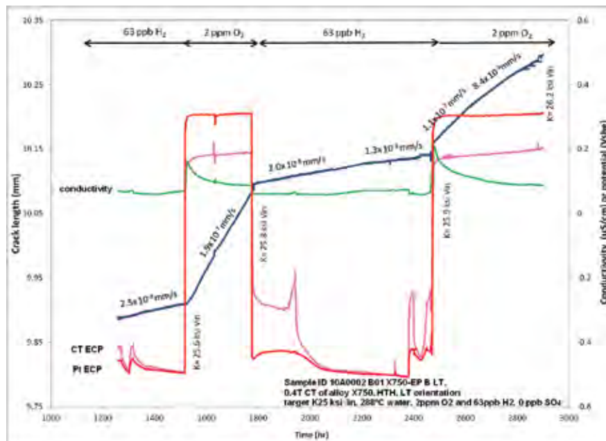
Figure 2. Typical baseline SCC test results for alloy X-750. CGR is the dark blue line.
