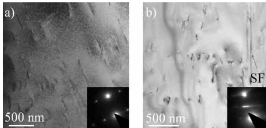
Figure 2. a) Brightfield TEM image near the (11-20) zone axis of ATR- \text{Ti}_3\text{AlC}_2 sample irradiated to 0.1 dpa at 100^\circ\text{C} reveals basal dislocations throughout the sample, some of which may possibly be short dislocation loops. b) TEM micrograph of same sample irradiated to 0.1 dpa at 500^\circ\text{C} taken in 2 beam condition tilted away from the (11-20) zone axis shows dislocation arrays parallel to the basal planes, as well as, stacking faults. Several of the dislocations do not appear straight due to the tilt of the sample, they are most likely curved within the basal planes. Further TEM investigation is needed to confirm the presence of dislocation loops or other irradiation induced defects within these materials.
