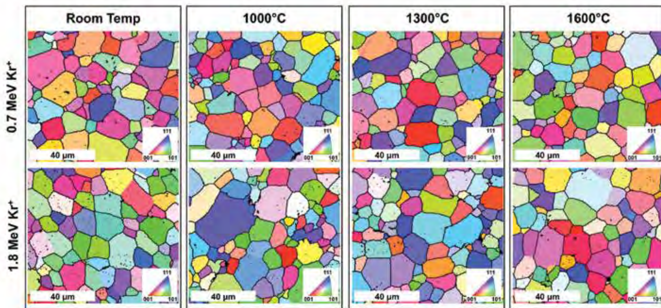
Figure 1. Representative EBSD maps of 0.7 MeV and 1.8 MeV Kr-irradiated \text{UO}_2 and the following post-irradiation anneal.
