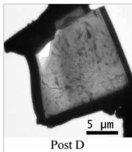
Figure 1. Three FIB-fabricated samples were prepared as shown in the micrograph left. The FIB lamellae at post B were lost due to handling and only lamellae from posts A (top right) and D (bottom right) were analyzed using ASTAR.
