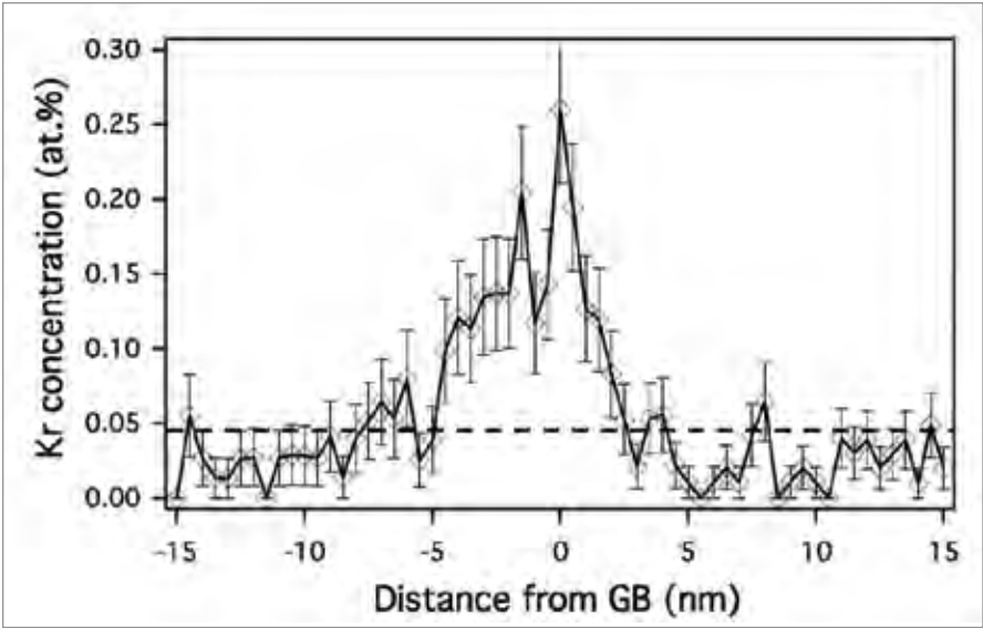
Figure 2. Kr concentration across a high angle grain boundary in \text{UO}_2 annealed at 1600^\circ\text{C} , showing significant segregation. The horizontal dashed line represents the bulk composition of Kr in the material.
