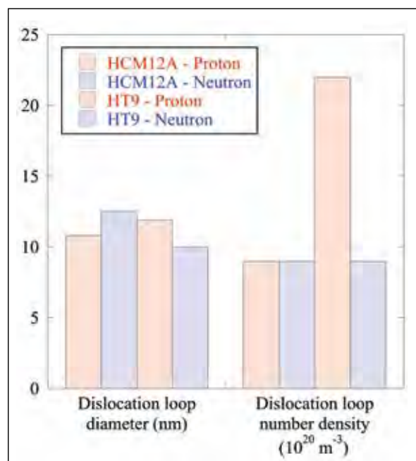
Figure 1. Irradiation-induced dislocation loop diameter and number density produced by proton and neutron irradiations to 3 dpa at 500°C in HCM12A and HT9.
