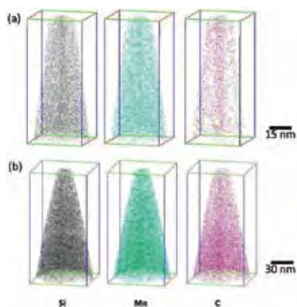
Figure 2. Representation of a three-dimensional (3D) reconstruction of CG low-carbon steel, (a) before and (b) after neutron irradiation by 3D atom-probe microscopy.
