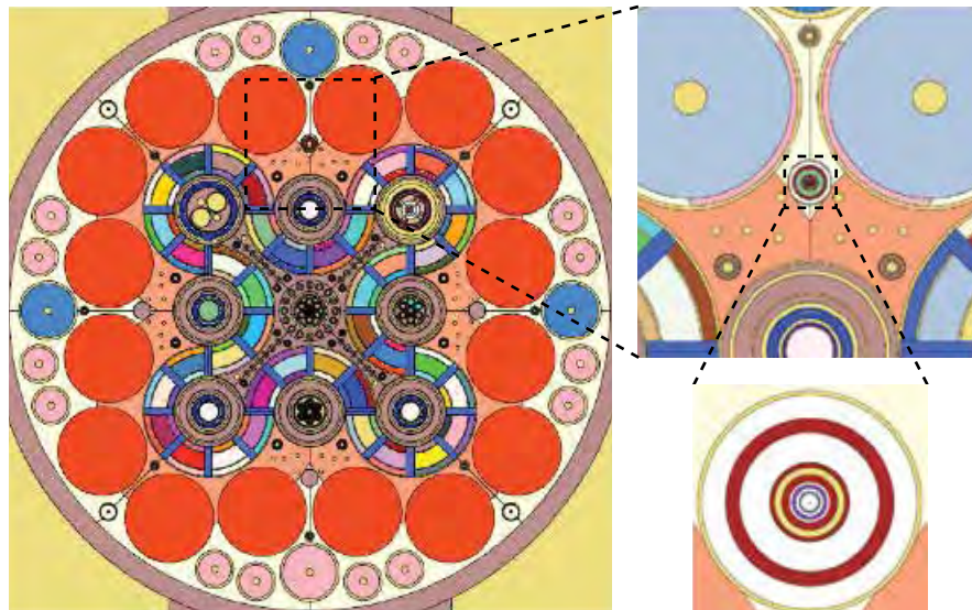
FIGURE 2. Details of the ATR MCNP model.
