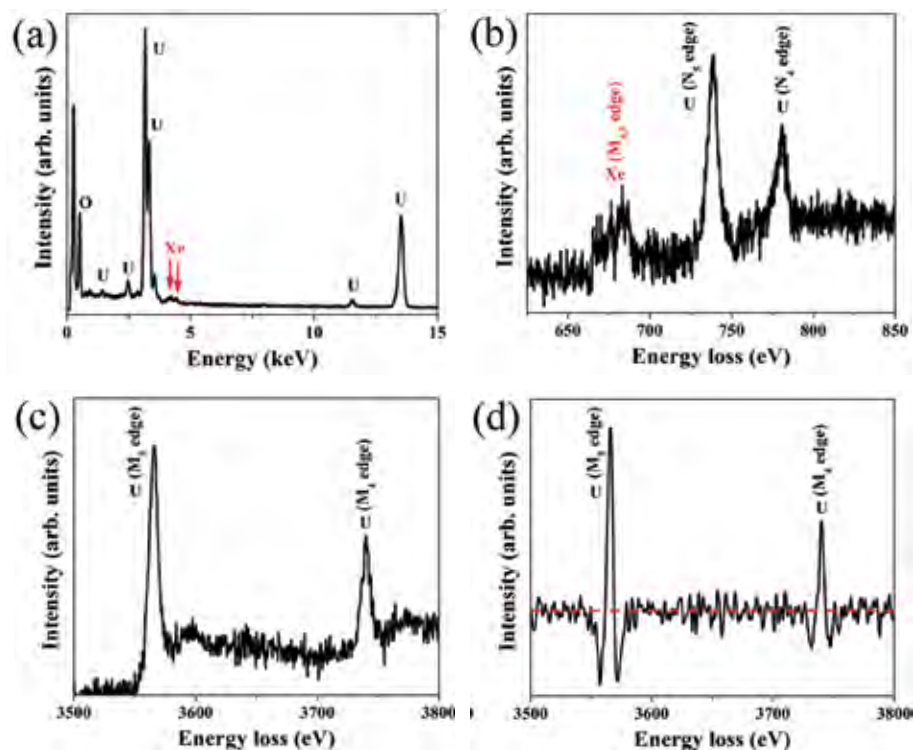
Figure 3. (a) Energy dispersive x-ray (EDX) and (b) and (c) EELS spectra of a \text{UO}_2 single crystal irradiated with 300 keV Xe at room temperature up to a dose of 1 \times 10^{16} ions/cm 2 . (d) The second derivative EELS spectrum of part (c).
