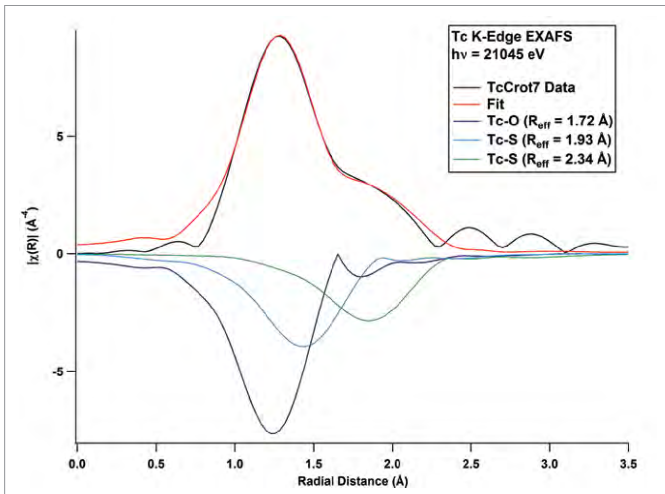
Figure 2. Fourier Transformation of the EXAFS spectra for the crotonic acid reaction.
