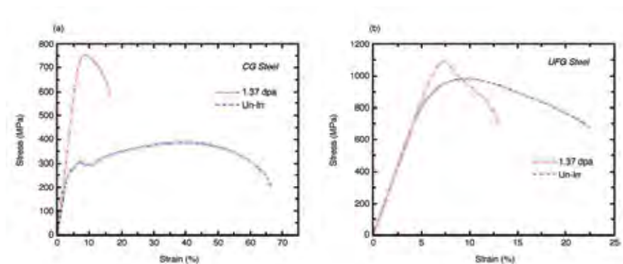
Figure 5. Engineering stress strain curves for (a) UFG and (b) CG before and after irradiation to 1.37 dpa.
