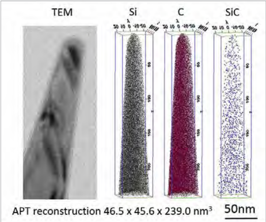
Figure 3. LEAP results showing the distribution of elements in a tip fabricated from surrogate Ag ion-implanted SiC.
