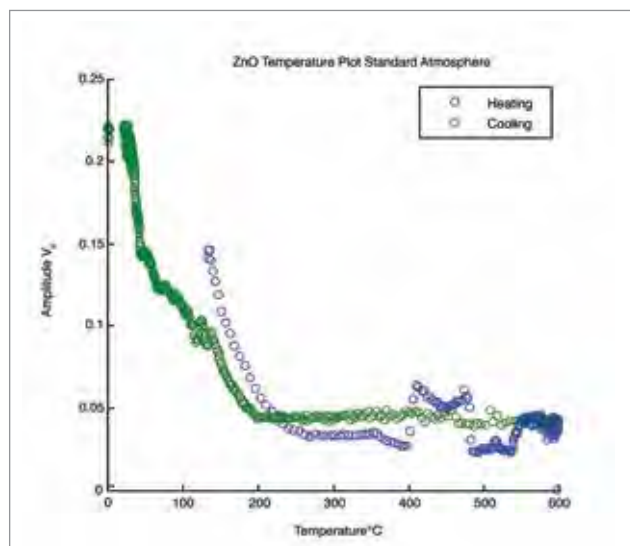
Figure 5. Temperature-dependent performance of the ZnO transducer. The transducer did not perform well at the design temperature, however it recovered its original amplitude upon cooling. This indicates that the sensor will operate satisfactorily during reactor shutdown, enabling us to measure performance degradation at those times.
