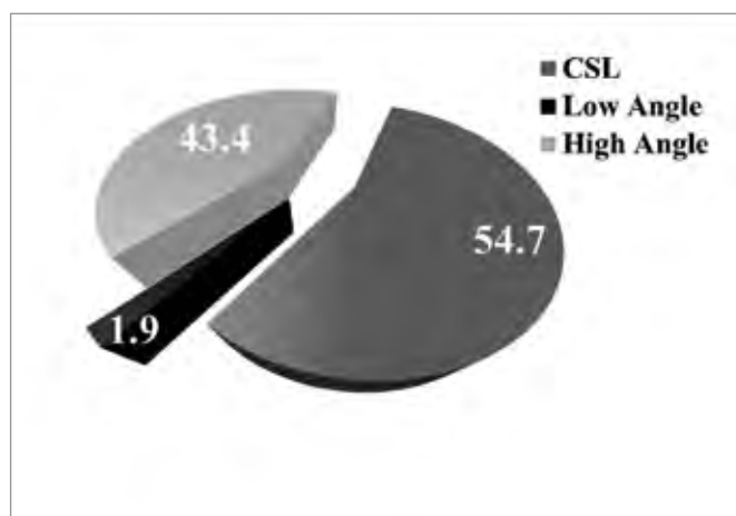
Figure 5. (a) Misorientation distribution of grain boundaries in Area B, sample IE, from particle AGR1-632-035. (b) A breakdown of grain boundary types [4].
