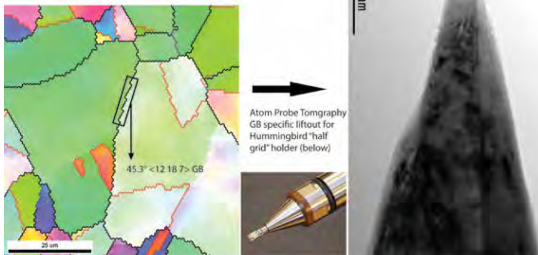
Figure 2. Highlight of EBSD map indicating a 45-degree grain boundary that is then thinned for a TEM and APT correlated study.
