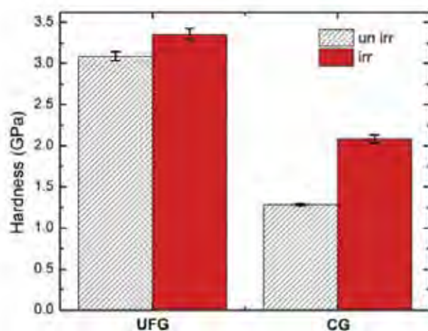
Figure 4. Micro hardness before and after irradiation for both UFG and CG low carbon steel
