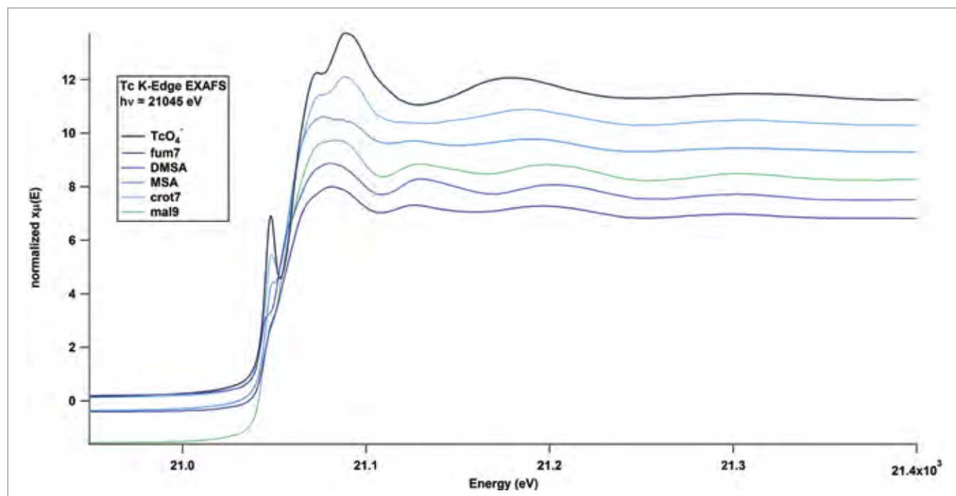
Figure 1. Tc K-edge EXAFS spectra of the standard complexes and experiment samples.
