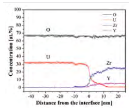
Figure 2. Atom probe 1-D concentration profile taken from the cylinder.
