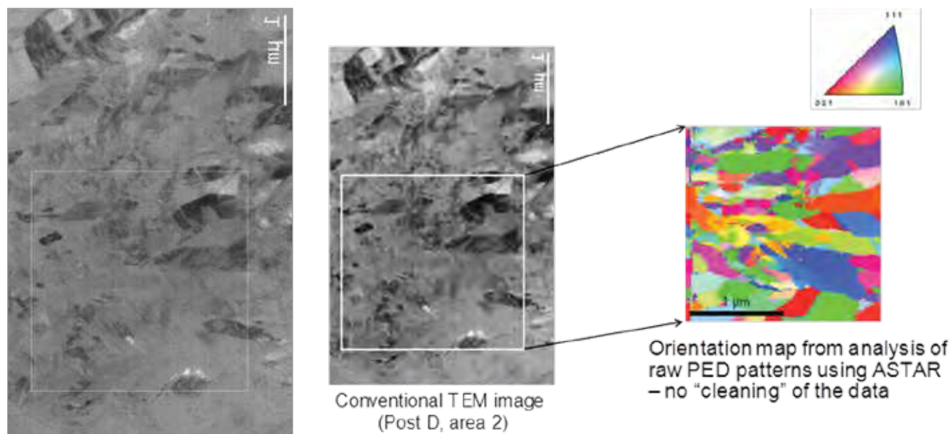
Figure 2. The crystallographic orientation of the area in the TEM image on the left is mapped on the right.
