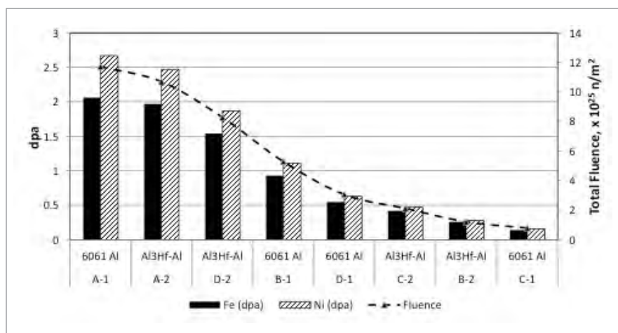
Figure 1. Calculated dpa values and total fluence for experiment.
