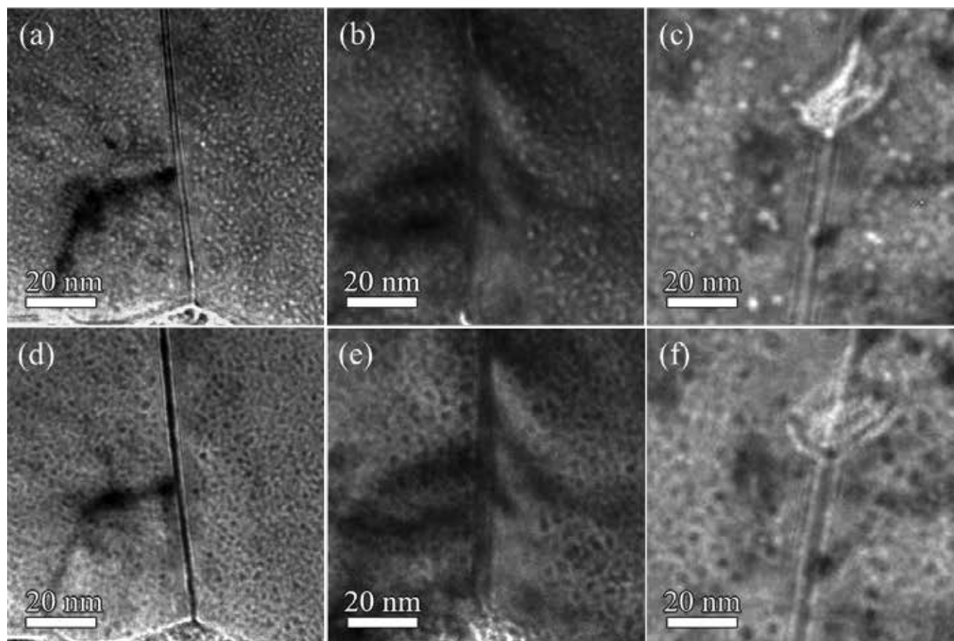
Figure 2. Cross-section TEM images showing bubbles near grain boundaries in Kr-irradiated, polycrystalline \text{UO}_2 after annealing at 1000°C (a and d), 1300°C (b and e), and 1600°C (c and f) for one hour. Figures a-c are under-focus images and Figures d-f are over-focus images.
