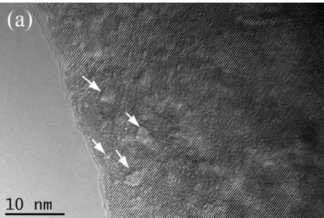
Figure 2. a) High-resolution TEM images of bubbles in a \text{UO}_2 single crystal irradiated with 300-keV Xe at room temperature at a dose of 5 \times 10^{14} ions/cm 2 . (b) An under-focus image of (a). Some bubbles are marked with arrows.
