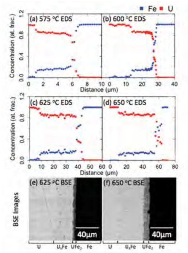
Figure 2. Concentration profiles obtained for diffusion couples U-Fe (single crystal) annealed at different temperatures (a-d) and typical BSE image at 625°C and 650°C diffusion couples showing formation of intermetallic crystals (e-f).
