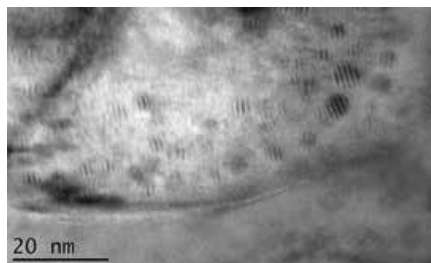
Figure 2. A TEM image of the 14LMT alloy specimen irradiated at 500°C/100 dpa.
