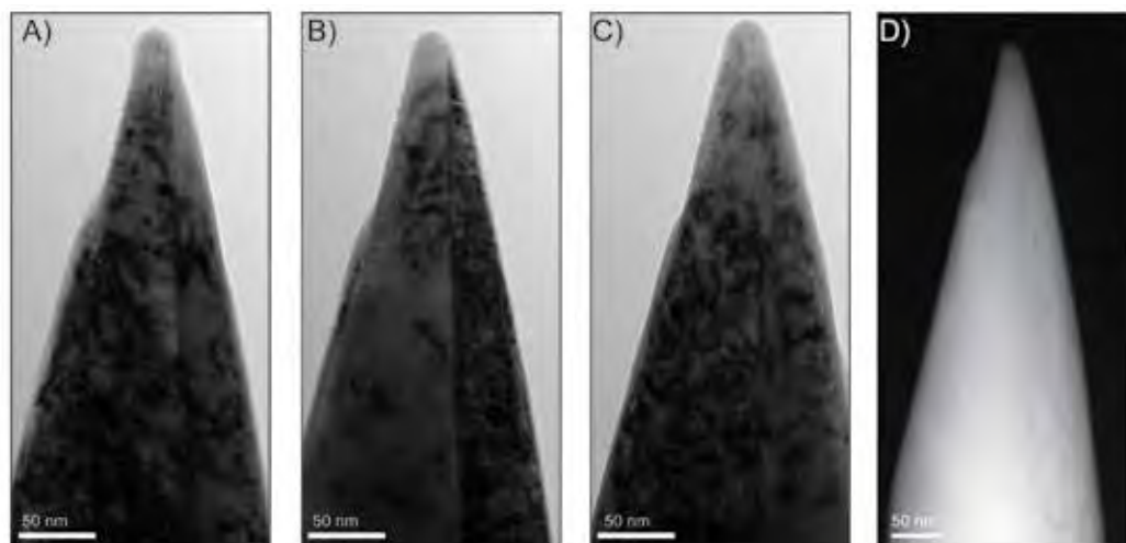
Figure 3. Sequence of three BF-TEM diffraction conditions (A-C) and STEM-HAADF (D) of the same GB structure shown in Figure 2.
