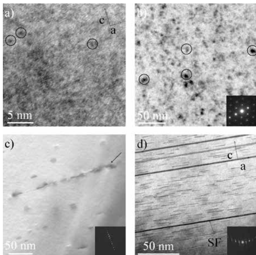
Figure 4: a) Brightfield high resolution transmission electron microscopy (HRTEM) micrograph of an edge on grain of a MITR- \text{Ti}_2\text{AlC} sample irradiated to 0.1 dpa at 360°C reveals perturbation of the basal planes and the presence of defect clusters and/or black spots (circled). b) TEM micrograph of a MITR- \text{Ti}_2\text{AlC} sample irradiated to 0.4 dpa at 360°C taken in 2 beam condition near the (0001) zone axis shows a higher density of small black spots (circled). c) Brightfield TEM micrograph of a fine-grained MITR- \text{Ti}_3\text{SiC}_2 sample irradiated to 0.1 dpa at 695°C shows dislocation loops imaged near the (11 -20) zone axis, parallel to the basal plane, agglomerating near a stacking fault (black arrow). The loops are seen as black and white lobes due to strain induced in the surrounding lattice, with an average defect density of 3.94 \times 10^{21} loops/ \text{m}^3 . d) Brightfield TEM micrographs of MITR- \text{Ti}_2\text{AlC} irradiated to 0.1 dpa at 695°C taken near the (11 -20) zone axis reveal dislocation loops edge on within the basal planes, with a higher average density of 1.1 \times 10^{23} loops/ \text{m}^3 .
