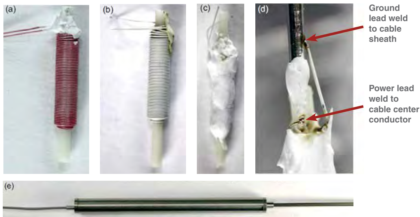
Figure 1. Magnetostrictive transducer fabrication. (a) Silver-palladium is wrapped around an alumina bobbin; (b) the wire is coated with a standoff insulation and heat treated; (c) the wire is coated with an alumina cement and heat-treated a second time; (d) leads are laser-welded to the coax cable and (e) welded into a pre-fabricated housing.
