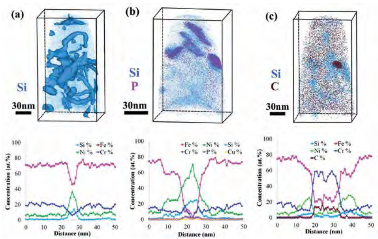
Figure 1. 3D reconstructions highlighting a) the network of dislocation loops segregated with Si and Ni as indicated by the concentration profile underneath. b) Phosphide plates with Ni and Si segregating to the plate interface, and c) small carbide and Ni_3Si precipitates with Ni and Si segregating to the carbide interface.
