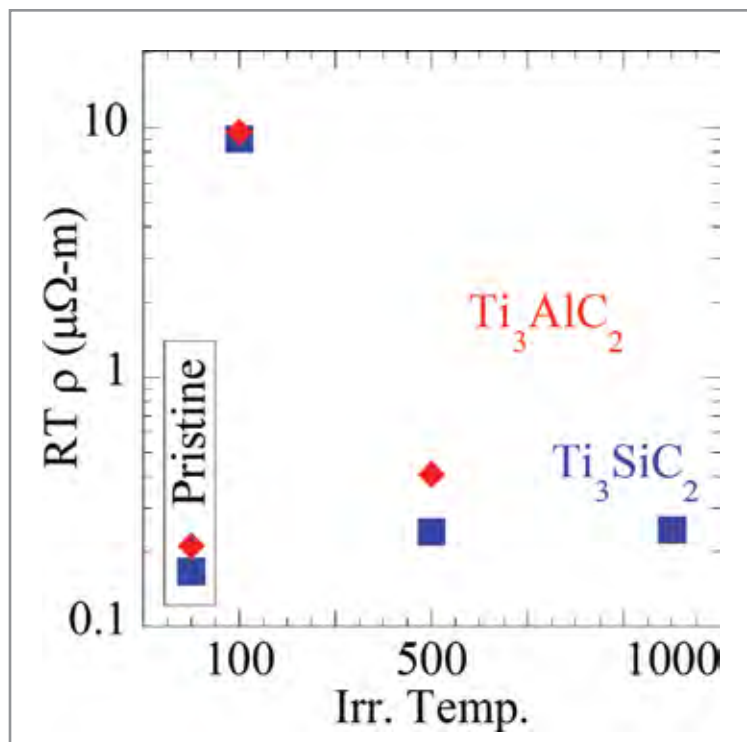
Figure 3. a) Room temperature resistivity plotted on a log scale as a function of neutron irradiation temperature at 0.1 dpa. After irradiation at 100°C, the resistivities of both \text{Ti}_3\text{SiC}_2 and \text{Ti}_3\text{AlC}_2 increase more than an order of magnitude. After irradiation at 500 and 1000°C, the resistivity of the \text{Ti}_3\text{SiC}_2 recovered to values near those of the pristine values. Some recovery is observed in \text{Ti}_3\text{AlC}_2 , with only a 2-fold increase after irradiation at 500°C.
