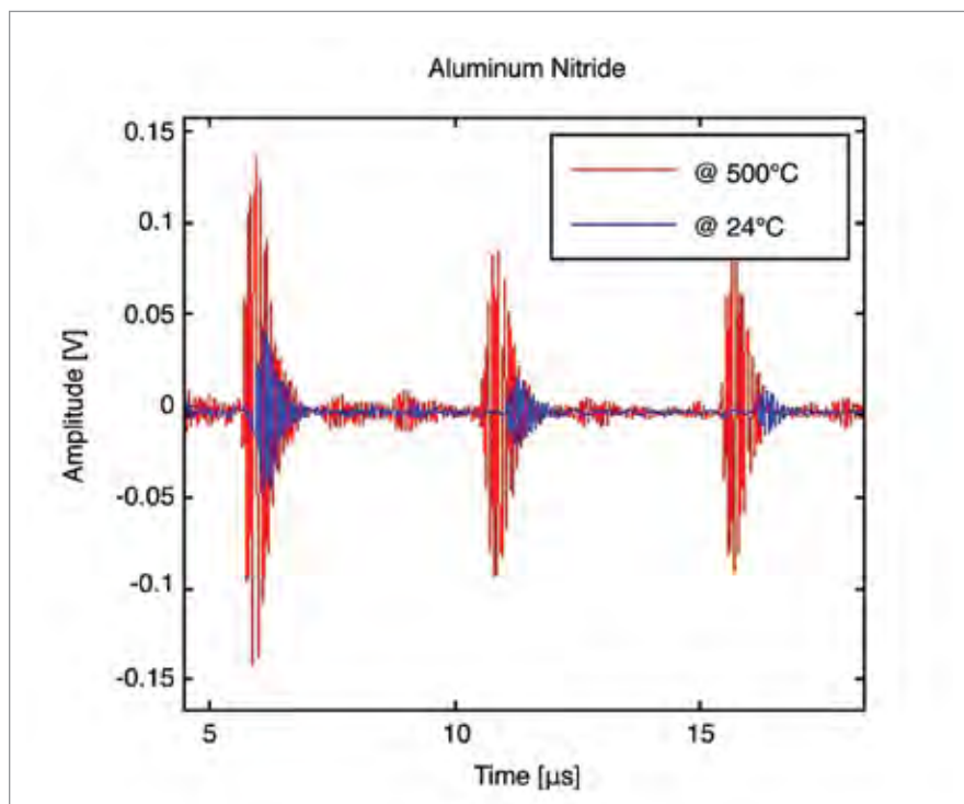
Figure 3. AlN ultrasonic pulse-echo amplitudes recorded at room temperature and at the irradiation temperature.
