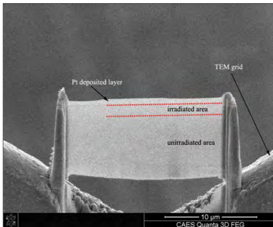
Figure 2. The FIB sample showing the Pt-deposited layer, irradiated and unirradiated areas.
