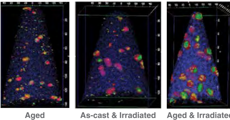
Figure 2. G-phase precipitates in aged, cast-irradiated, and aged-irradiated CF-3. Image sizes reflect identical scales, and the blue dots represent Cr atoms. The concentrations of the iso-surface plots of Mn, nickel (Ni), and silicon (Si) are 5, 20, and 15 at.%, respectively.
