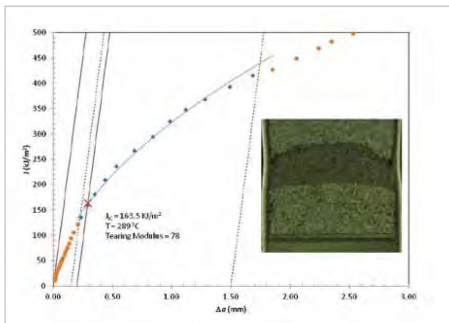
Figure 3. Typical fracture toughness test results for alloy X-750 at elevated (289°C) temperature.
