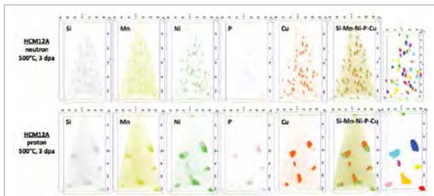
Figure 2. LEAP tip reconstructions of neutron- (top) and proton-irradiated (bottom) HCM12A to 3 dpa at 500°C, showing (left to right) Si, Mn, Ni, P, Cu; Si-Mn-Ni-P-Cu; and cluster identification.
