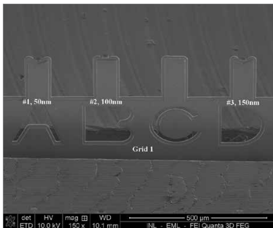
Figure 1. Three FIB-fabricated samples were prepared as shown in the micrograph left. The FIB lamellae at post B were lost due to handling and only lamellae from posts A (top right) and D (bottom right) were analyzed using ASTAR.
