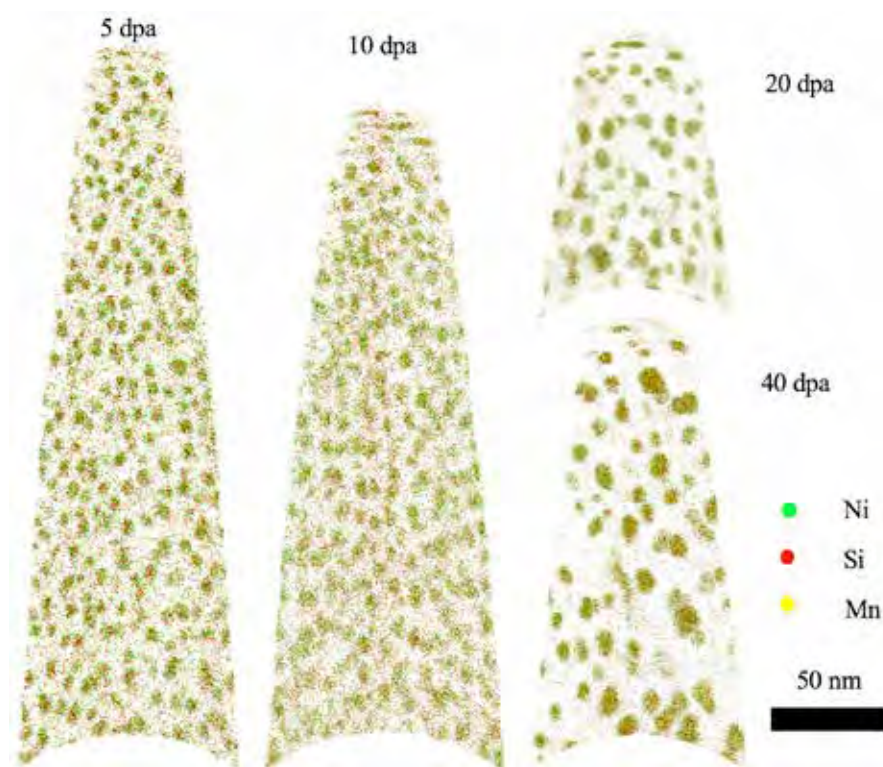
Figure 3. Ni-Si-Mn clusters in the irradiated ferrite phase.
