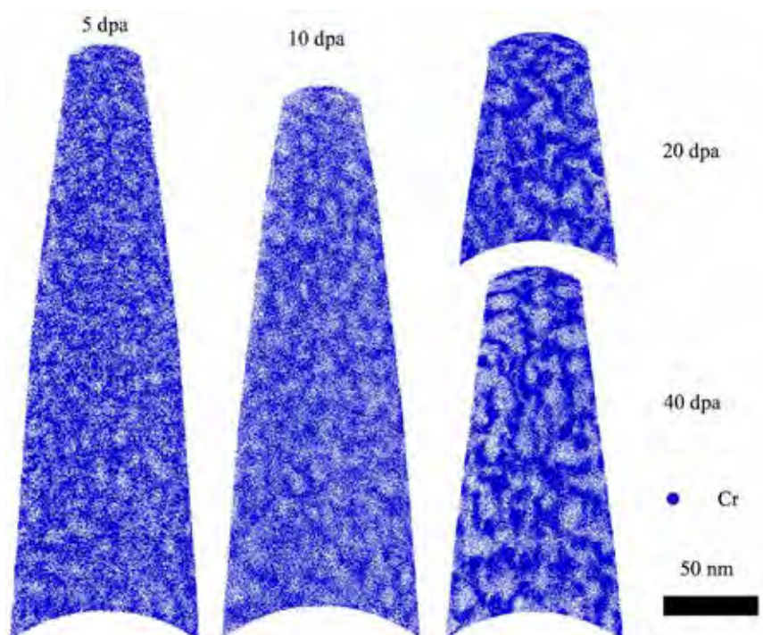
Figure 1. Spinodal decomposition in the ferrite phases of CF3 Cast Stainless Steel irradiated to 5, 10, 20 and 40 dpa, respectively.
