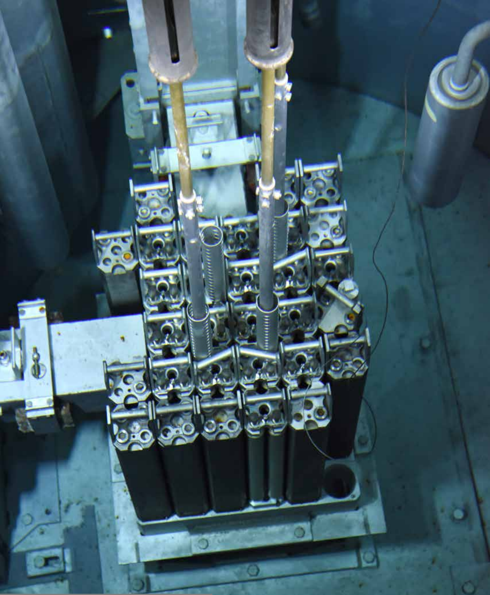
Neutron Radiography Reactor (NRAD), MFC, INL
