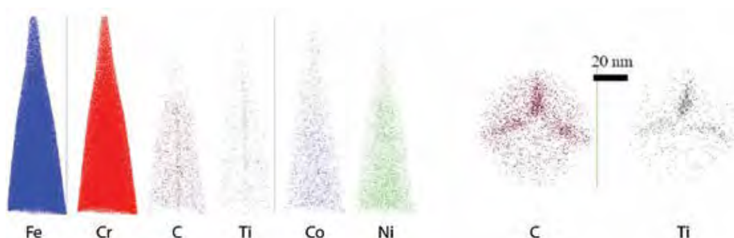
Figure 2. Atom probe tomography of tempered martensite in as-received Fe-9Cr alloy. Enrichment of carbon and titanium in the grain boundary were obtained.
