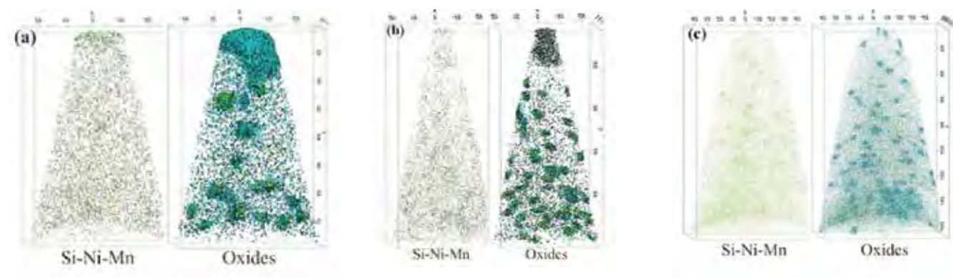
Figure 1. Atom probe tomography (APT) reconstructed tips showing Si-Ni-Mn clustering on oxide nanoparticles in model Fe-9Cr irradiated with (a) 5 MeV Fe ++ , 100 dpa, 400°C, (b) 2 MeV protons, 3 dpa, 500°C, and (c) neutrons in ATR, 3 dpa, 500°C.
